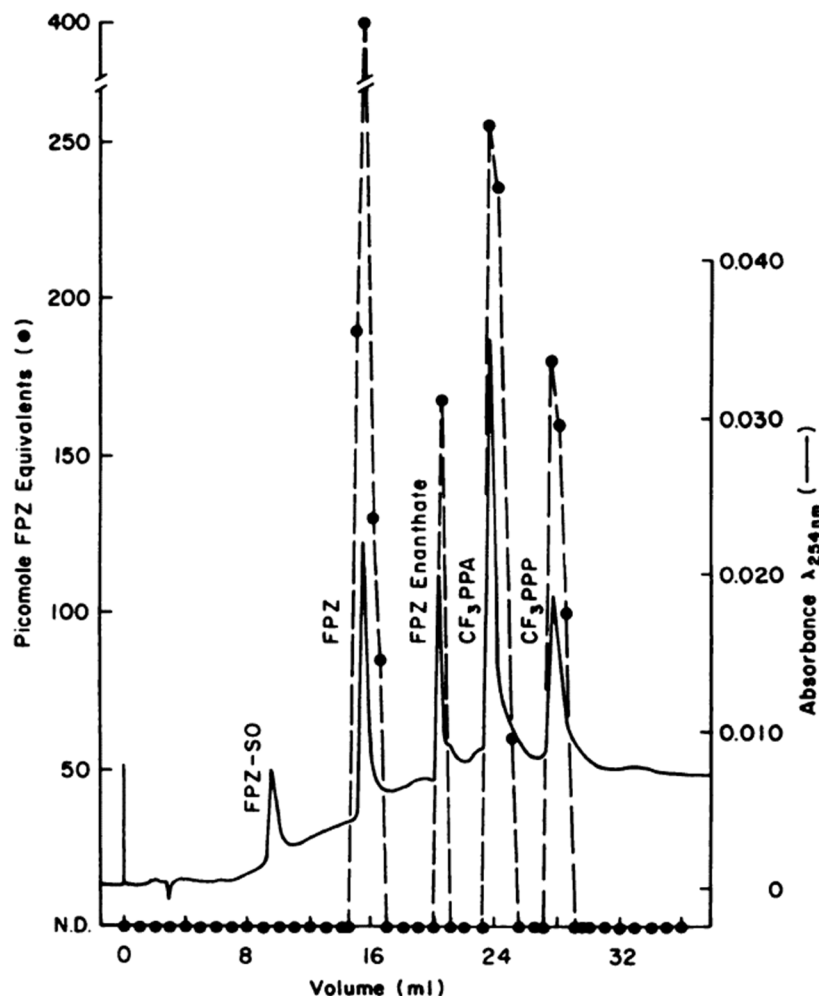
Fig. 2. HPLC-RIA analysis \langle \bullet \rangle with spectral trace (-) , of FPZ and four of its derivatives. A solution (50 \mu\text{l} ) containing FPZ (0.82 nmol), FPZ-SO (0.80 nmol), FPZ enanthate (0.45 nmol), CF 3 PPA (1.20 nmol) and CF 3 PPP (0.52 nmol) was applied to the column. Fractions of eluent were collected, lyophilized, reconstituted in horse serum buffer and analyzed by the RIA, as described under "Materials and Methods." N.D. signifies less than 0.37 pmol of FPZ equivalents. Elution volumes are not identical to those reported in table 1 because a different C 18 - \mu Bondapak column and a linear gradient (70 to 100% methanol/0.01 M sodium phosphate, pH 7.4 at 25°C) was used. Although absolute elution volumes vary with different C 18 - \mu Bondapak columns, the relative pattern of elution of a parent compound and its derivatives remains unaltered.
