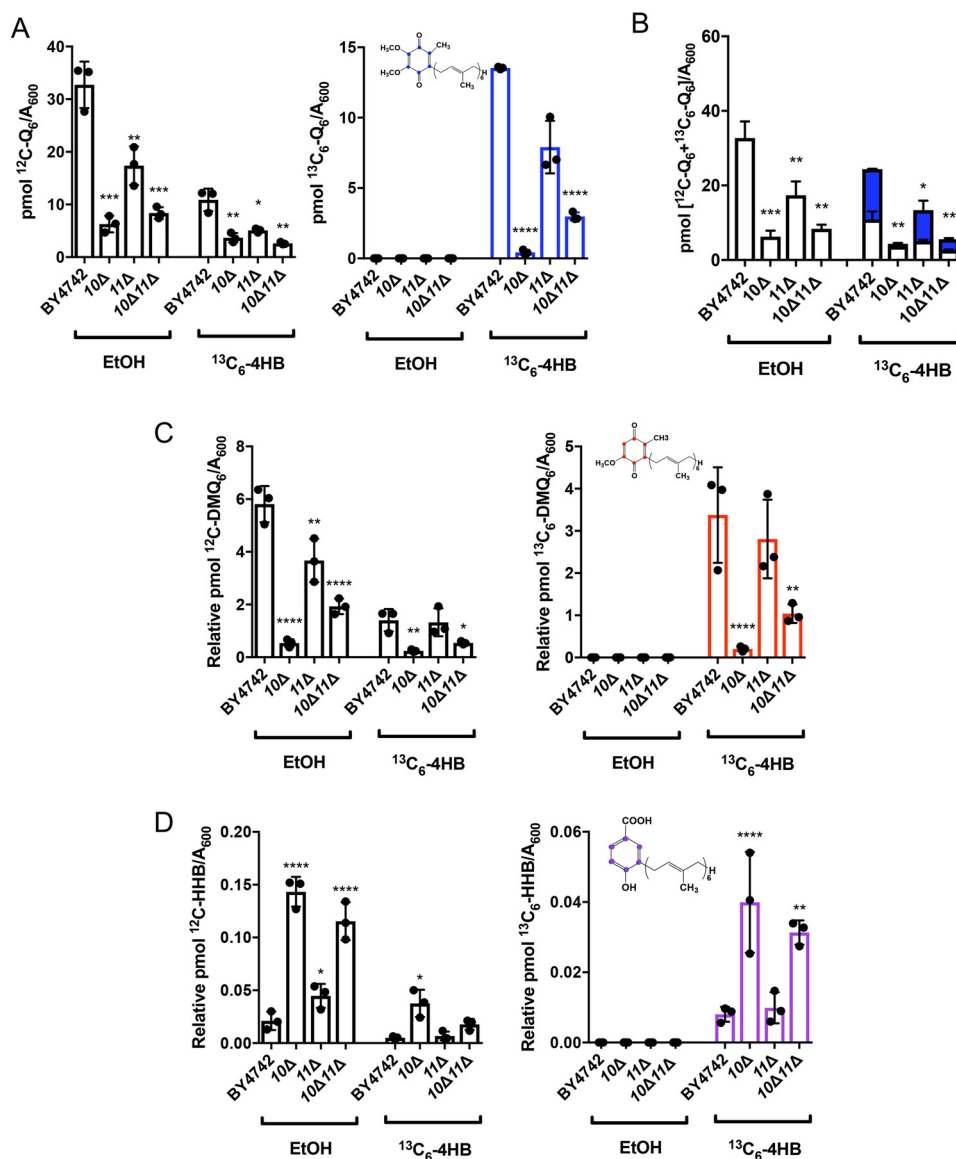
Figure 4. Low amounts of de novo ^{13}\text{C}_6\text{Q}_6 in whole-cell lipid extracts of the coq10Δ mutant are only partially restored by deletion of COQ11 . Triplicates of 6-ml cultures in YPGal were labeled at A_{600} \sim 1 with 5 \mu\text{g/ml} ^{13}\text{C}_6\text{4HB} or EtOH vehicle control, and 5 ml of each culture were collected after 4 h, lipid-extracted, and analyzed by LC-MS/MS. A , unlabeled ^{12}\text{C}_6\text{Q}_6 and de novo -synthesized ^{13}\text{C}_6\text{Q}_6 (blue); B , total amount of \text{Q}_6 determined from the sum of ^{13}\text{C}_6\text{Q}_6 and ^{12}\text{C}_6\text{Q}_6 ; C , ^{12}\text{C}_6\text{DMQ}_6 and ^{13}\text{C}_6\text{DMQ}_6 (red); and D , ^{12}\text{C}_6\text{HHB} and ^{13}\text{C}_6\text{HHB} (purple) were measured from the whole-cell lipid extracts of WT and the coq10Δ , coq11Δ , and coq10Δcoq11Δ mutants. Values are the mean of three replicates. The data show mean \pm S.D., and the statistical significance as compared with WT is represented by *, p < 0.05 ; **, p < 0.001 ; and ****, p < 0.0001 .
