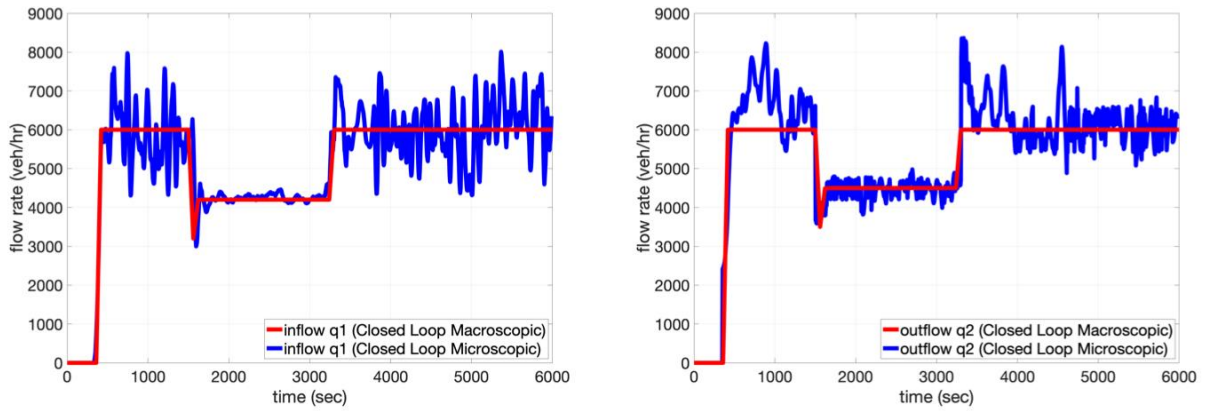
Figure 100. Macroscopic/Microscopic Behavior of q1 & q2 of the Closed-loop System
