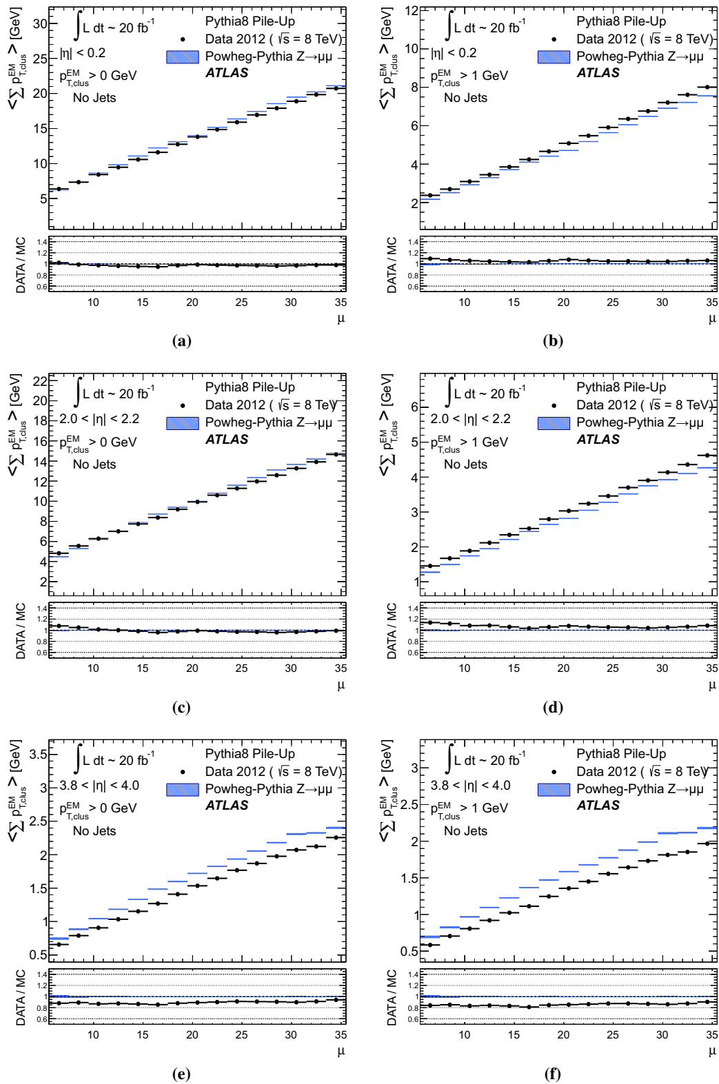
Fig. 24 The average transverse momentum flow ( \langle \sum p_{T,clus}^{EM} \rangle ) evaluated as function of the pile-up activity measured by the number of proton–proton interactions per bunch crossing \mu , in several calorimeter regions. In a , c , and e , \langle \sum p_{T,clus}^{EM} \rangle(\mu) is shown in the central ( |\eta| < 0.2 ), end-cap ( 2.0 < |\eta| < 2.2 ), and the forward ( 3.8 < |\eta| < 4.0 ) region, respectively, using topo-clusters with p_{T,clus}^{EM} > 0 . The corresponding results
