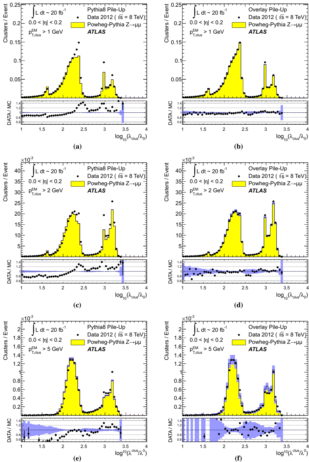
Fig. 29 The distribution of the topo-cluster depth location, measured in terms of \log_{10}(\lambda_{\text{clus}}/\lambda_0) , for selected topoclusters within |\eta_{\text{clus}}| < 0.2 and with a transverse momentum p_{T,\text{clus}}^{\text{EM}} , evaluated on the EM scale, larger than various thresholds. Results are shown for an inclusive Z \rightarrow \mu\mu event sample recorded in 2012. Data are compared to distributions from MC simulations including fully simulated pile-up for
