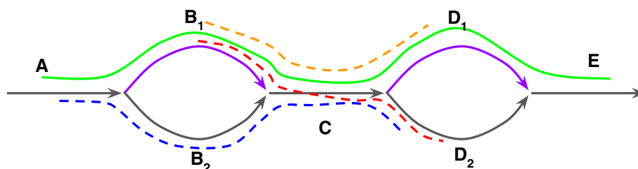
Fig. 9 Examples of conflicting and non-conflicting gene paths in an assembly graph. Purple edges B_1 and D_1 are classified as unique but black edges B_2 and D_2 are classified as non-unique since they are shorter than the minLength threshold. Edges A, C, and E are classified as non-unique because their indegrees and/or outdegrees prevent their classification as unique edges. The green path conflicts with the red path but does not conflict with the blue and yellow paths. Purple edges represent unique edges of the green contig-path
