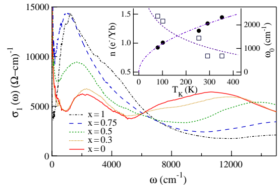
Fig. 1. Main Panel: The optical conductivity of \text{YbIn}_{1-x}\text{Ag}_x\text{Cu}_4 . Inset: The peak frequency \omega_0 and the integral of \sigma_1(\omega) from \omega = 40 – 4000\text{ cm}^{-1} plotted against T_K .
