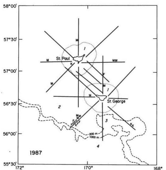
FIG. 4. Survey effort during 22 July–17 August 1987. For keys to numbered regions, see Figure 1 caption. Tracklines shown were daytime surveys. F = fin whale sighting, K = killer whale sighting, M = minke whale sighting.
