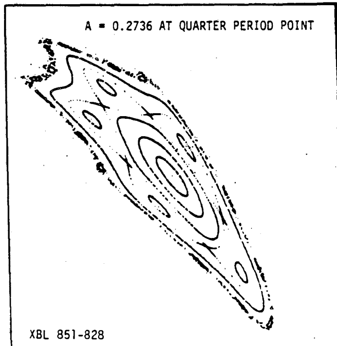
Fig. II.2 Phase plot for the runs of Fig. 1, plotted at Z = \pi/2 \bmod 2\pi . Scales: Horizontal: -2.0 to 2.0 , for x ; Vertical: -0.6 to 0.6 , for x' .
