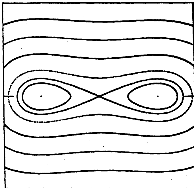
Fig. III.16. T = -0.11126 . De-Vogelaere Variables. Scales: 0.4852 to 0.4860; \pm 0.000001 . After the second bifurcation (leading to Order-16 fixed points), one of the (now unstable) Order-8 fixed points develops horizontal loops, that contain stable Order-16 fixed points. The fixed points shown are 2/8: 0.485601872680, 0. 4/16: 0.485356977954, 0, 0.485849305665, 0. XBL 851-861
