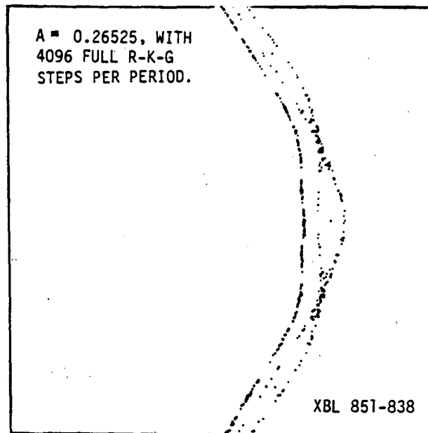
Fig. II.7a Detail related to Fig. II.7 ( A = 0.26525 ); Scales:
