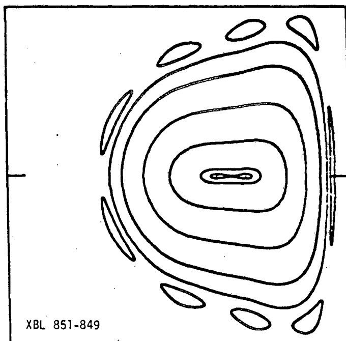
Fig. III.4 T = -0.1034 . De-Vogelaere Variables. Scales: 0.48 to 0.56; \pm 0.0025 . Enlarged view of bifurcation.
