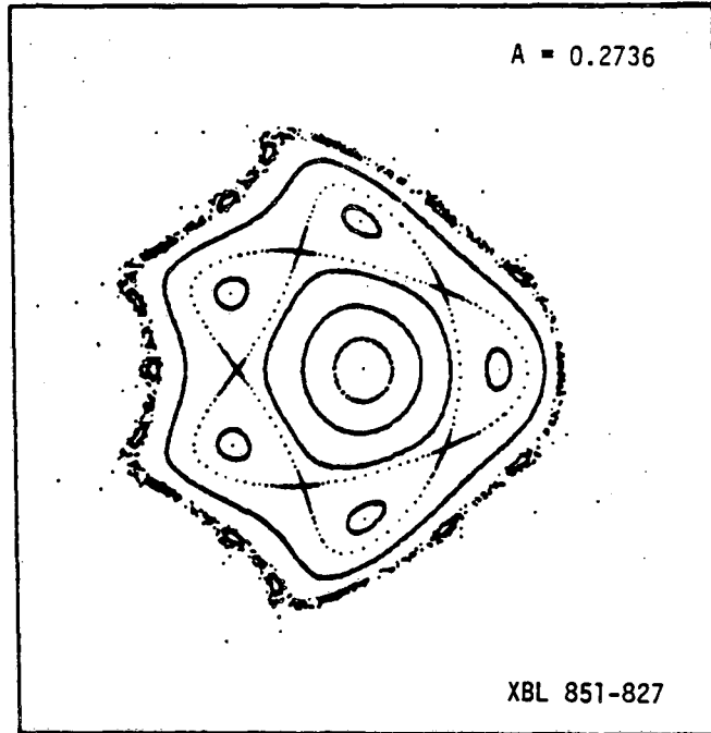
Fig. II.1 x' vs. x phase plot, at Z=0 \bmod 2\pi , for solutions to Eqn. (1) with A = 0.2736 ( \sigma_0 \approx 74.59 deg.) to the scales:
