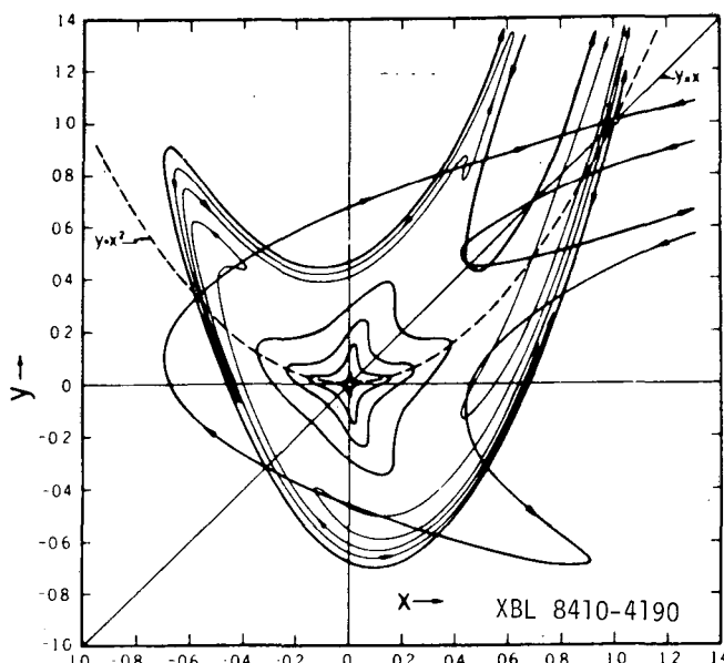
Fig. 1.3 A partial extension of the curves of Fig. 1.2, showing "tentacles" reaching off the figure and "worms" in the interior. Since the entrance channel for the "worms" becomes very narrow, the figure becomes difficult to draw completely as the iteration progresses. Some apparently closed curves around the stable fixed point at x = 0, y = 0 are also shown. The peculiar behavior near the origin seems less mysterious if one recalls that the function y = 1/2f(x) approaches the limit of zero slope, where the curve degenerates to four points, and where the slightest perturbation can cause a slow migration about the center and a concomitant slow change in radius.
