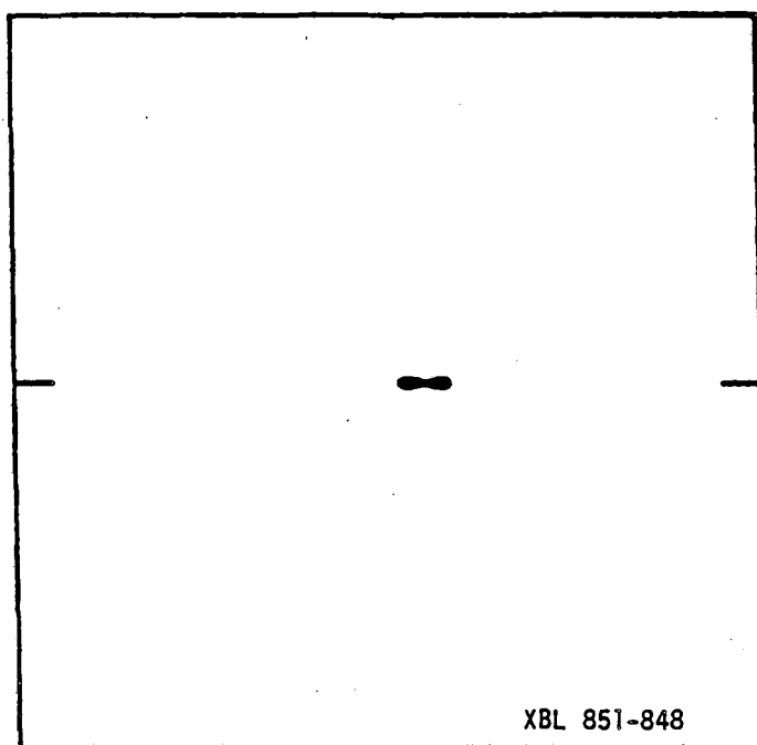
Fig. III.3 T = -0.1034 . De-Vogelaere Variables. Scales: 0.45 to 0.60; \pm 0.003 .
