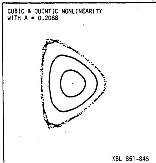
Fig. II.9a Detail related to Fig. II.9, for Eqn.(2) with A = 0.2088 , Scales:
