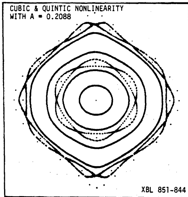
Fig. II.9 Phase plot, at Z = 0 \bmod. 2\pi , for solutions to Eqn. (2) with A = 0.2088 ( \sigma_0 = 55.1621 deg.). Scales:
