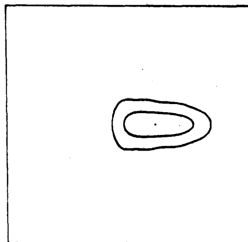
Fig. III.22 A = 0.2651 6th order fixed point is stable.
