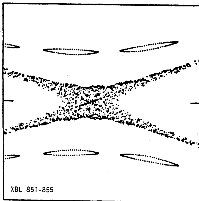
Fig. III.10. T = -0.1045 . De-Vogelaere Variables. Scales: 0.53 to 0.54; \pm 0.001 . Detail -- to emphasize stochastic region about the unstable fixed point at x = 0.534416773867 .
