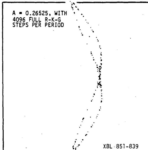
Fig. II.7b Detail related to Fig. II.7 ( A = 0.26525 ); Scales:
