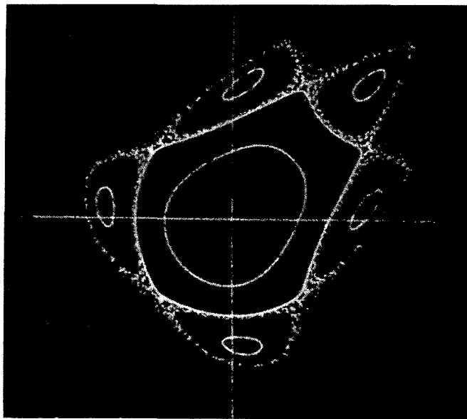
Fig. 1.4. Apparently smooth phase curves and a scattering of points resulting from iteration of the Hénon-Froeschlé transformation, with \cos \alpha = 0.22 and coordinates x, y appropriate to expressing the transformation in the McMillan form. Five islands of stability (containing stable fixed points of order 5) are seen surrounding the area associated with the order-1 fixed point at the origin. The outermost smooth curve, shown as bounding this inner area, resulted from the starting values X_0 = 0.5350, Y_0 = 0 (Froeschlé notation), and the scattered points result from X_0 = 0.5375, Y_0 = 0 . Scale (as indicated by the coordinate axes): -1.0 to 1.0. XBB 840-7763
