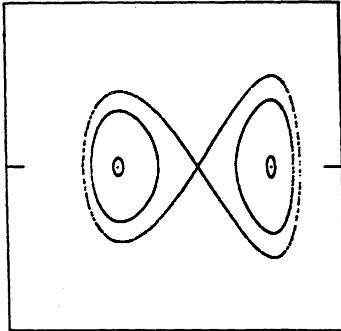
Fig. III.17. T = -0.11223 . De-Vogelaere Variables. Scales: 0.4965 to 0.4990; \pm 0.000002 . After the third bifurcation (leading to Order-32 fixed points), one of the (now unstable) Order-16 fixed points develops horizontal loops, that contain stable Order-32 fixed points. The fixed points shown are 4/16: 0.497936225267, 0. 8/32: 0.497335279454, 0, 0.498484243334, 0. XBL 851-862
