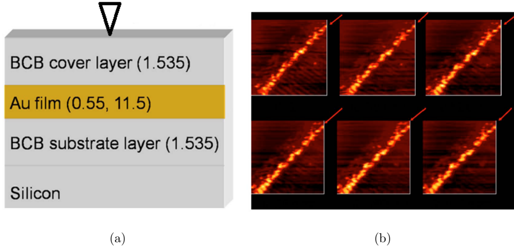
Figure 5.6: NSOM experiment on LRSP imaging from [95]. (a) Experimental setup, with solid dielectric layer on either side of Au film. (b) Optical intensity distribution recorded by NSOM for various tip heights from 0 to 1000 nm. Because the tip sits atop a solid dielectric, the NSOM actually records far-field scattering rather than near-field evanescent waves. Both images adapted from [95].
