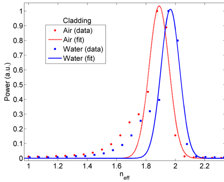
Figure 4.10: Integrated Fourier transform of the complex field with scan lines removed (1 for air overlcladding, 2 for water overlcladding) to reduce spectral leakage. This leaves a low-index tail visible which is the remnant of the suppressed peak.
