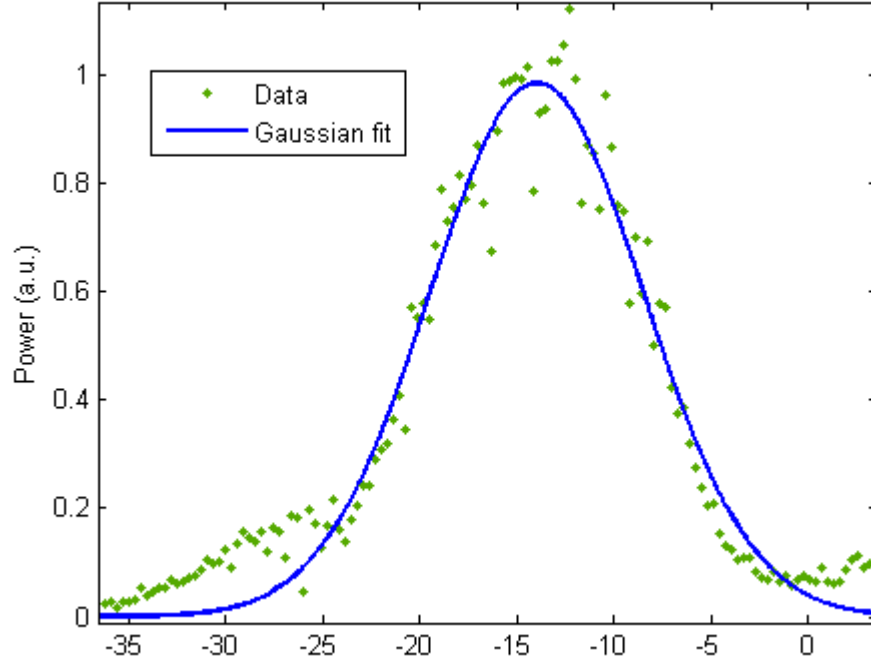
Figure 5.13: Transverse distribution of the LRSP mode with Gaussian fit. Fit has FWHM=12.9\mu m , with R^2 > 95\% .
