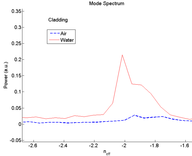
Figure 4.13: Backward-propagating mode due to Fresnel reflection ( \sim 1\% intensity). Applying the Fourier transform to the complex field allows separation of negative and positive frequencies.
