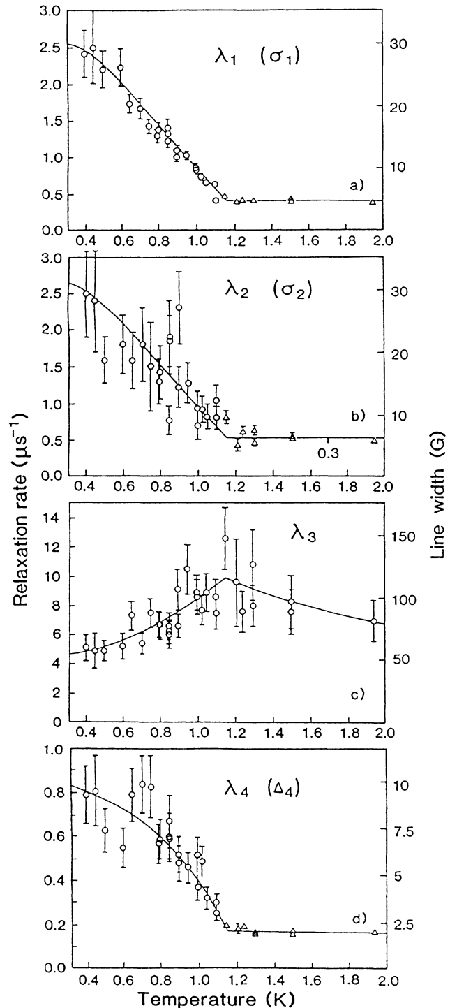
FIG. 3. Temperature dependence of the \mu^+ relaxation rates associated with frequencies (a) \nu_1 , (b) \nu_2 , (c) \nu_3 , and (d) \nu_4=0 . The solid lines are guides to the eye (see text for details).
