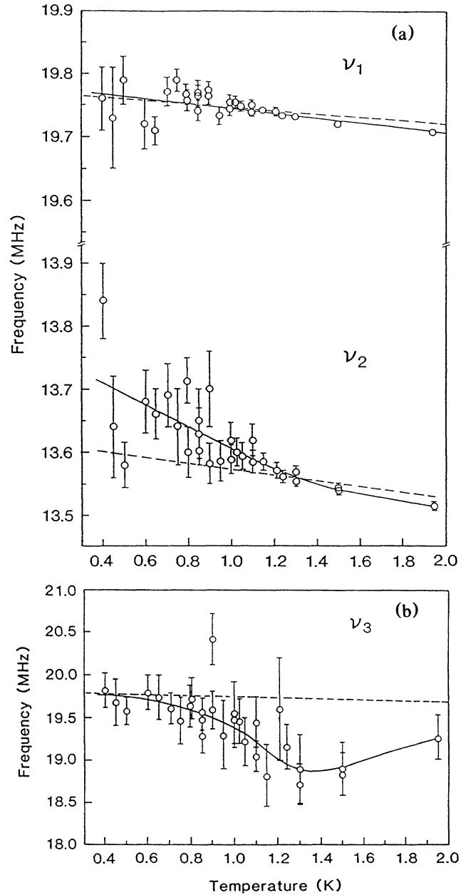
FIG. 2. Temperature dependence of the \mu^+ -spin precession frequencies (a) \nu_1 and \nu_2 and (b) \nu_3 . The dashed lines in (a) represent the earlier data of Ref. 4; the dashed line in (b) the present \nu_1 values. The solid lines are guides to the eye.
