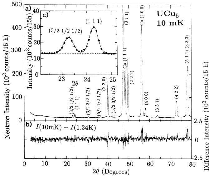
FIG. 1. (a) Neutron-diffraction pattern at T=10 mK. The neutron wavelength is 1.703 Å. The solid lines are guides to the eye. (c) A blup of the magnetic (\frac{3}{2} \frac{1}{2} \frac{1}{2}) reflection next to a nuclear peak. (b) Difference neutron diagram I(10 \text{ mK}) - I(1.34 \text{ K}) .
