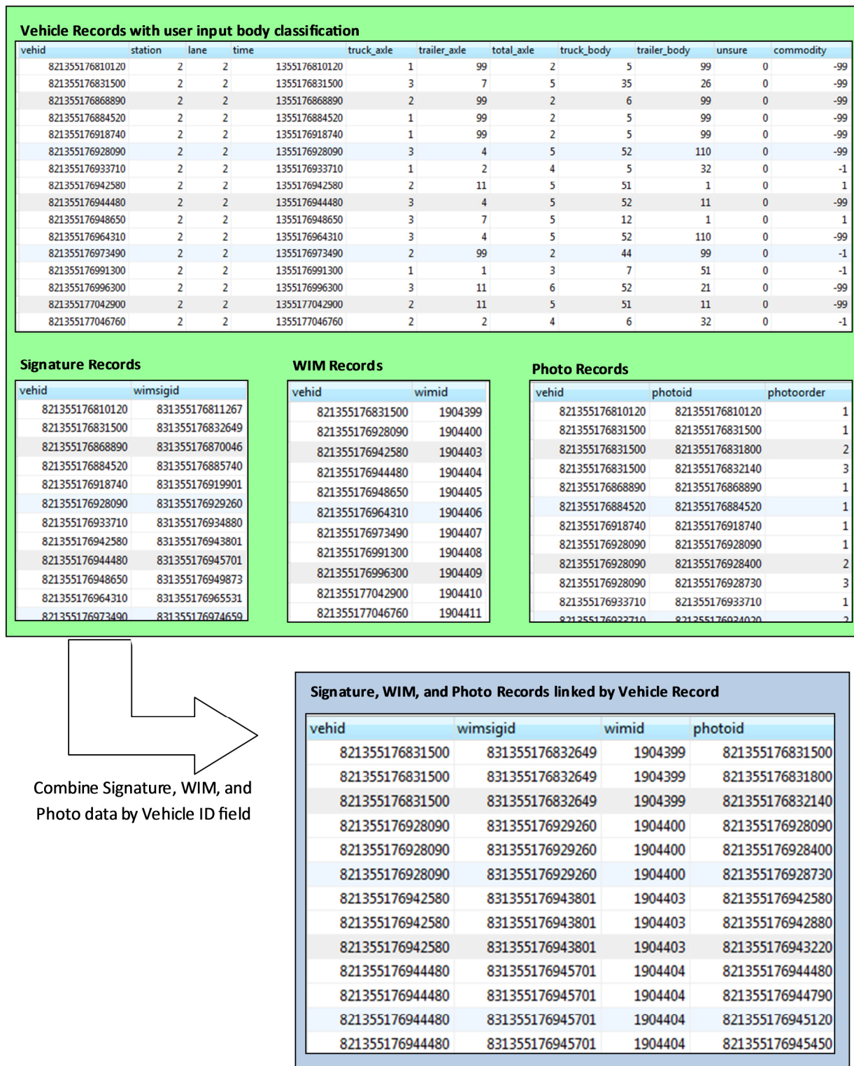
Figure 3.12 Database Structure for Data Groundtruth
