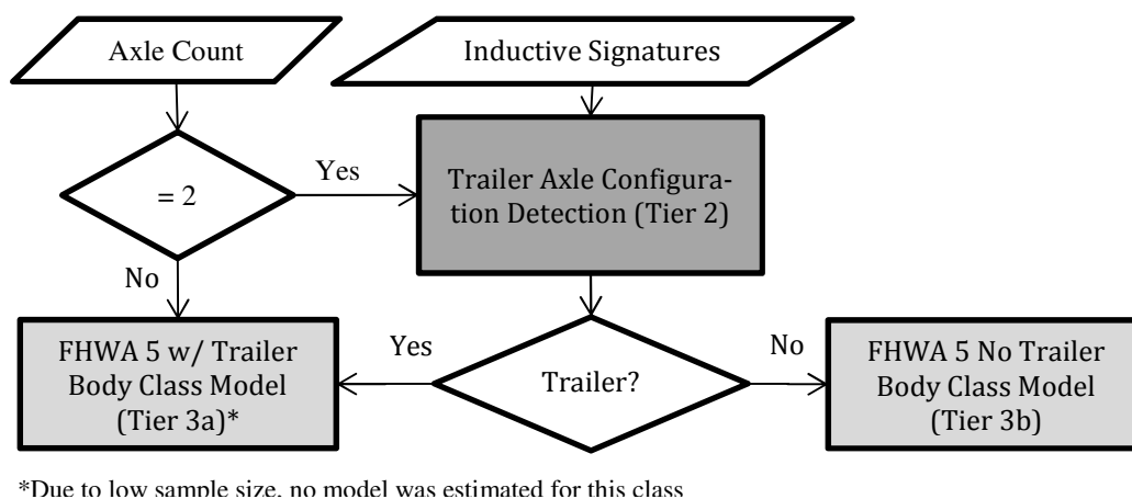
Figure 5.13 FHWA Class 5 Model Framework
