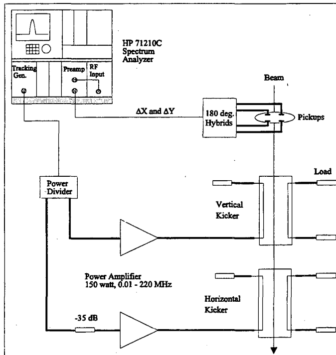
Fig. 2 Block diagram of fractional tune measurement system.
