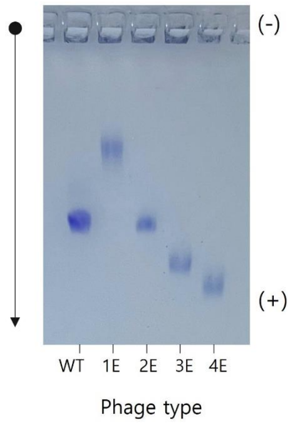
Figure 3-18. Gel electrophoresis measurements for WT- and engineered-phages.
