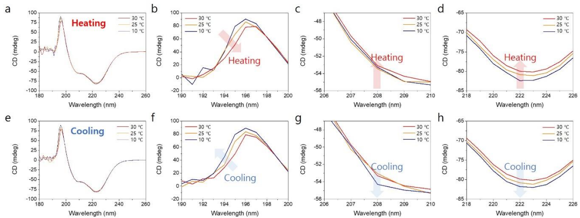
Figure 4-21. CD spectra of the M13 phage. (a) Changes in the CD signal during the heating process. (b-d) CD spectra at specific wavelength regions (193, 208, and 222 nm), revealing a decrease in the \alpha -helical structural feature of the pVIII protein. (e) The CD signal during the cooling phase. (f-h) CD spectra at typical wavelength regions (193, 208, and 222 nm), illustrating a restoration of the \alpha -helical structural characteristic of the pVIII protein to its initial state. These findings indicate a reversible structural transformation. Reprinted with permission. 3 Copyright 2023, John Wiley and Sons.
