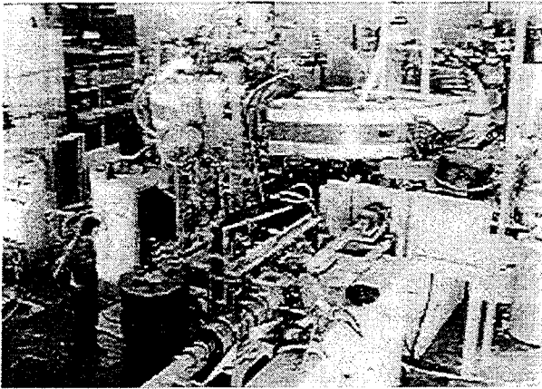
Figure 9. ADONE, the first of the large e^+e^- storage rings. One can see that significant space had been provided for particle experiments. The figure shows the ring during construction; operation commenced in 1969. (Photograph from the personal collection of Andrew M. Sessler.)
