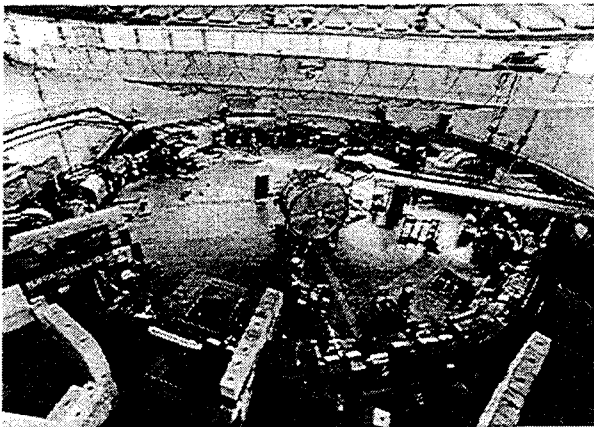
Figure 8. The first Soviet e^-e^+ storage ring, VEPP II. Each beam had 700 MeV and in 1967 it was used to study electron-positron annihilation into pions at the rho resonance. This was the first experiment ever using an e^-e^+ storage ring. (Photograph from the personal collection of Andrew M. Sessler.)
