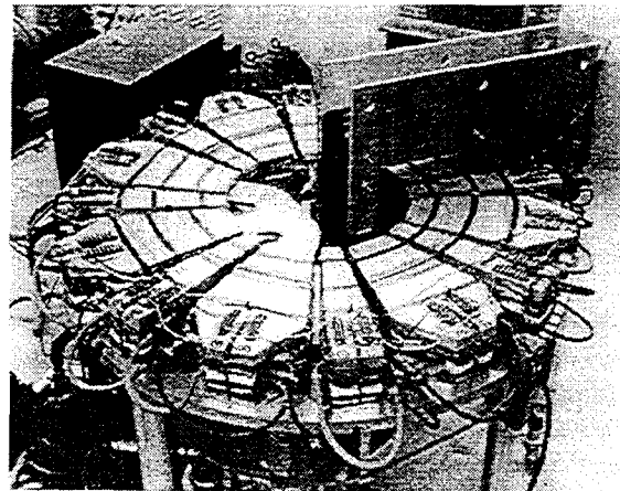
Figure 1. The Mark 1 Model built by the MURA Group in Michigan in 1955. There are 8 sectors, and electrons of 30 keV were injected at a radius of 34 cm and accelerated, by betatron action (note the large core), to 400 keV at a radius of 50 cm. (Photograph from the personal collection of Andrew M. Sessler.)
