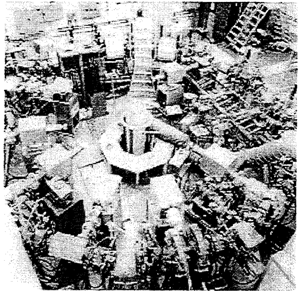
Figure 4. The CERN Electron Model for the ISR, initiated in 1960. The circumference is 24m, including 12 straight sections each 1m long. The electron energy could be 100 MeV, but 2 MeV was used for most studies. (Photograph courtesy of CERN.)
