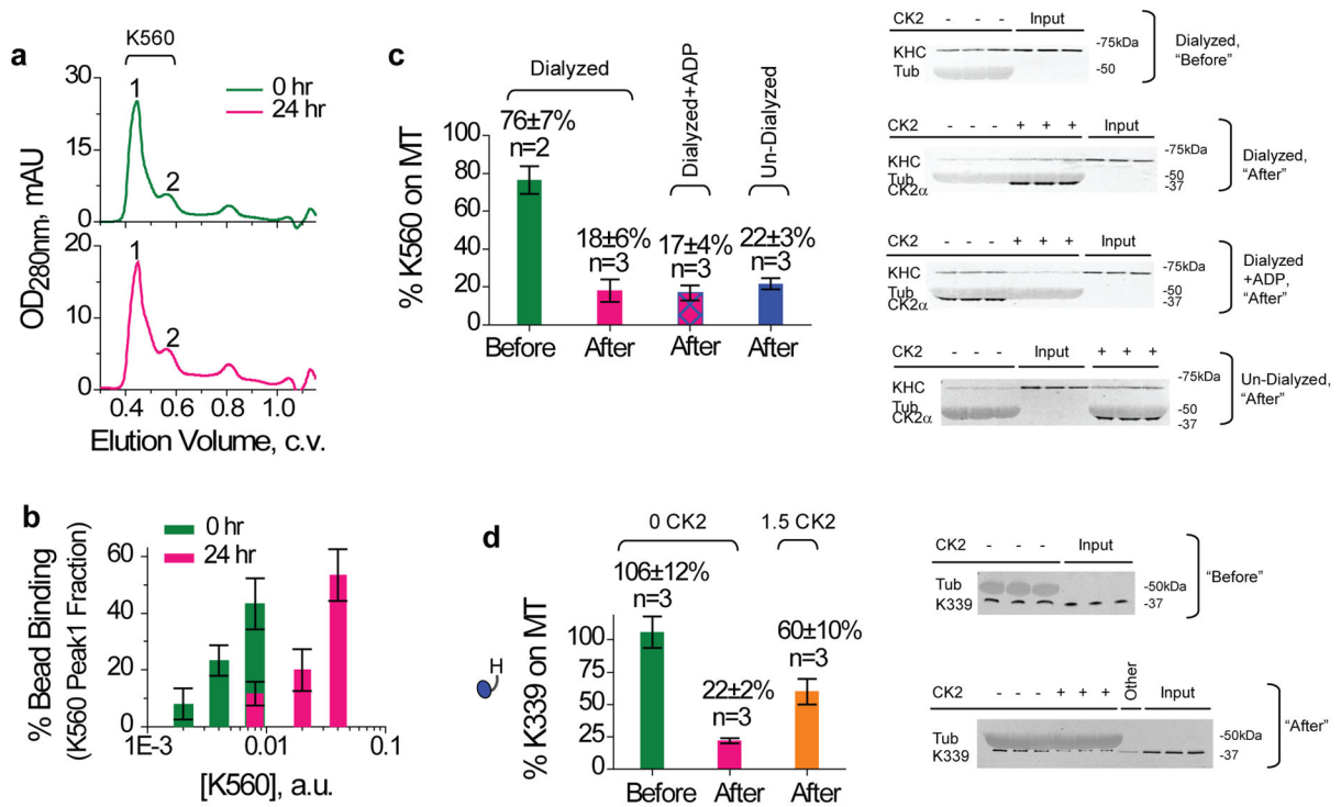
Figure 7. Mechanism studies of K560 inactivation. Values are mean±SEM, sample sizes n are indicated. (a–b) Role of oligomerization. The oligomerization state (a) and activity (b) of K560 immediately after Ni purification (0 hr), and after a 24 hr ice incubation (24 hr). (a) Size exclusion chromatography using Superdex-200. K560 content was verified by Coomassie (not shown) and bead assay (b) . Peak positions 1 and 2 were well correlated with the dimeric and monomeric forms of Eg5-513-GFP analyzed using the same column 43 . Relative abundance of peak 1 vs. 2 was 4.73±0.86 at 0 hr, and 4.4±0.43 at 24 hr (mean±data range, n=2 each). (b) Motor activity in peak 1 elute, analyzed by bead assay (n~30) at 1mM ATP. When compared at the same motor concentration per bead, ~5-fold less K560 dilution was required to reach the same bead binding fraction at the 0 th hr. (c) Role of nucleotide-bound state. The fraction of K560 competent for microtubule-binding at 4mM AMPPNP, before and after an 1.5hr incubation on ice, assayed by immunoblot against kinesin heavy chain (AKIN01). Cross reactivity of the polyclonal antibody AKIN01 with tubulin (‘Tub’) is used for loading reference. Input reference lanes are as indicated (‘Inputs’). Ni-purified K560 was dialyzed against 5mM EDTA to deplete bound nucleotide, and then supplemented with 10mM Mg 2+ (‘Dialyzed’) or 10mM Mg 2+ /10 mM ADP (‘Dialyzed+ADP’). Controls used un-dialyzed K560 undergoing identical ice incubation (‘Un-Dialyzed’). The effect of CK2 during incubation is quantified later in text. We hypothesize that an additional freeze-thaw cycle may contribute to the increased magnitude of inactivation observed in (c) vs. (b) . (d) Role of head-head interaction. Co-sedimentation of K339 monomer with microtubules at 4 mM AMPPNP, assayed by immunoblot against kinesin heavy chain (AKIN01). Cross reactivity of AKIN01 with tubulin (‘Tub’) was used for loading reference. Shown are microtubule pull-downs using Ni-purified K339 immediately after thawing (‘Before’), or
