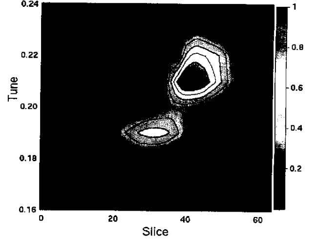
Figure 4: WARP simulation, Tune vs. Z position, averaged over turns 100–200 after injection. 94.4 ps/sample, positive Z is towards the tail of the bunch (later in time).
