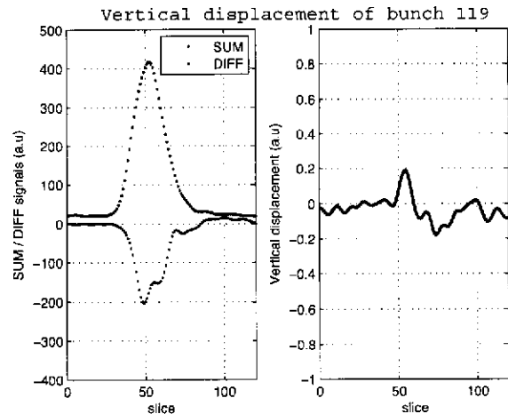
Figure 1: Sum and DeltaY signals from SPS receiver (after equalization). Bunch 119, turn 100 after injection, 26 GeV. The vertical offset is removed in the rightmost plot. Bunch 119 is becoming unstable, as seen in the high-frequency structure. Each slice (sample) is 20 ps.
