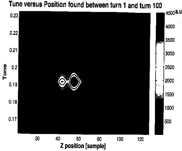
Figure 2: Tune vs. Z position, bunch 119, averaged over turns 1–100 after injection. 20 ps/sample, Positive Z is towards the tail of the bunch (later time).
