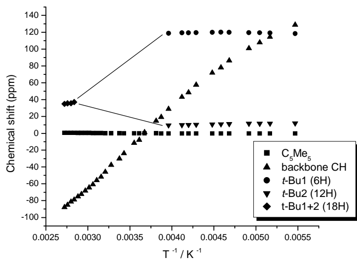
Figure 10. Chemical shift ( \delta ) vs. T^{-1} plot of the ^1\text{H} NMR resonances of (\text{C}_5\text{Me}_5)_2\text{Yb}(\text{dad}(\text{H})\text{-}t\text{-Bu}) in \text{toluene-}d_8 at temperatures from -70 to +90^\circ\text{C} .
