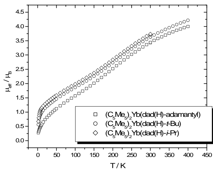
Figure 4a. \mu_{\text{eff}} vs. T plot of (\text{C}_5\text{Me}_5)_2\text{Yb}(\text{dad}(\text{H})\text{-alkyl}) compounds
