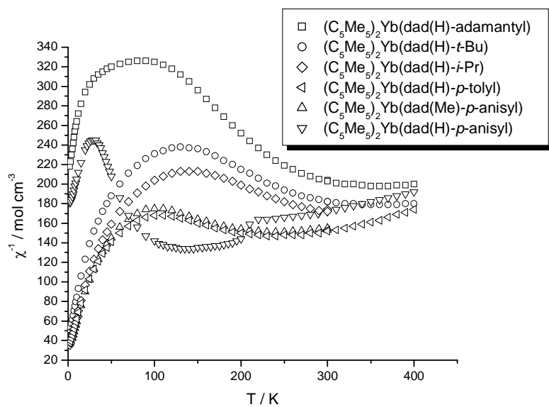
Figure 3. \chi^{-1} vs. T plot of (\text{C}_5\text{Me}_5)_2\text{Yb}(\text{dad}(\text{R}')\text{-R}) compounds
