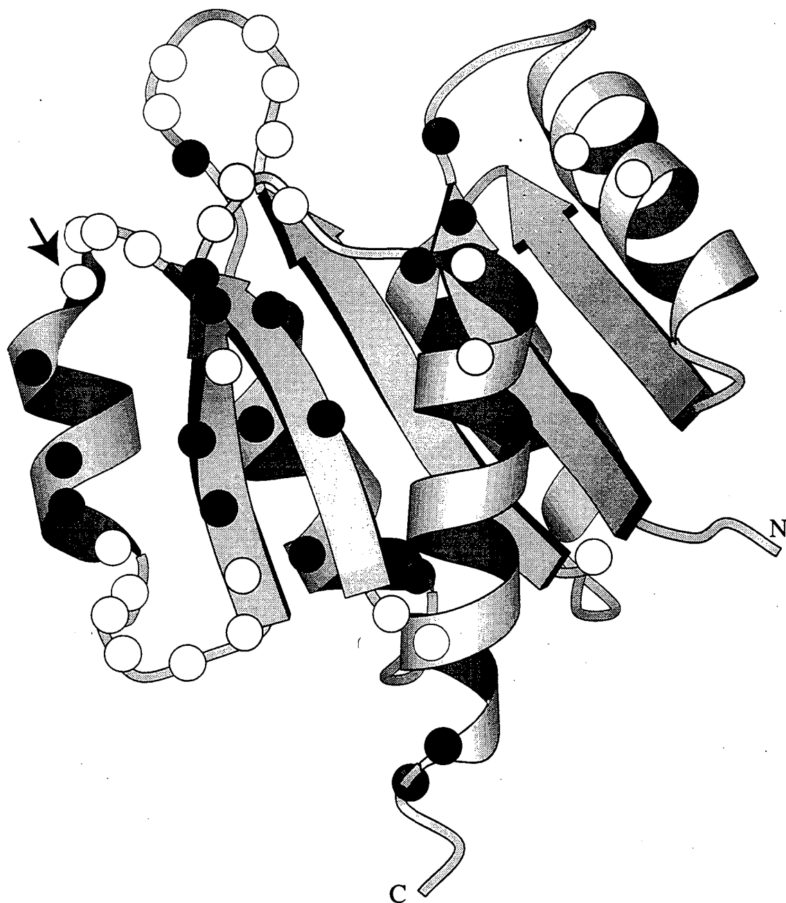
Figure 5.6: The largest chemical shift differences between D86N and wildtype NTRC mapped onto the structure of wildtype NTRC. The black spheres represent residues which have moved at least 50 Hz. The white spheres represent residues for which either amide was not detectable or the assignments for both D86N NTRC and wildtype NTRC were not obtained. The arrow indicates the site of mutation.
