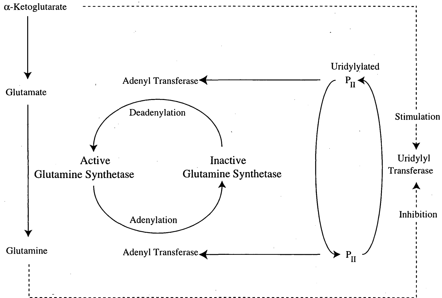
Figure 2.4: Diagram of the post-translational control of the activity of glutamine synthetase.
