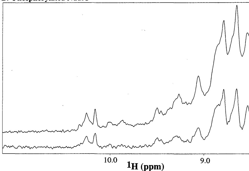
Figure 4.4: 1D ^1\text{H} 1-1 spin echo spectra of unphosphorylated NTRC (0.5 mM NTRC, 200 mM phosphate buffer pH 6.8) and phosphorylated NTRC (0.5 mM NTRC, 200 mM phosphate buffer pH 6.8, 300 mM carbamyl phosphate, 27 mM \text{Mg}^{2+} ) with a relaxation period of 0.1 ms (upper spectrum) and 5.1 ms (lower spectrum). Details are given in the text.
