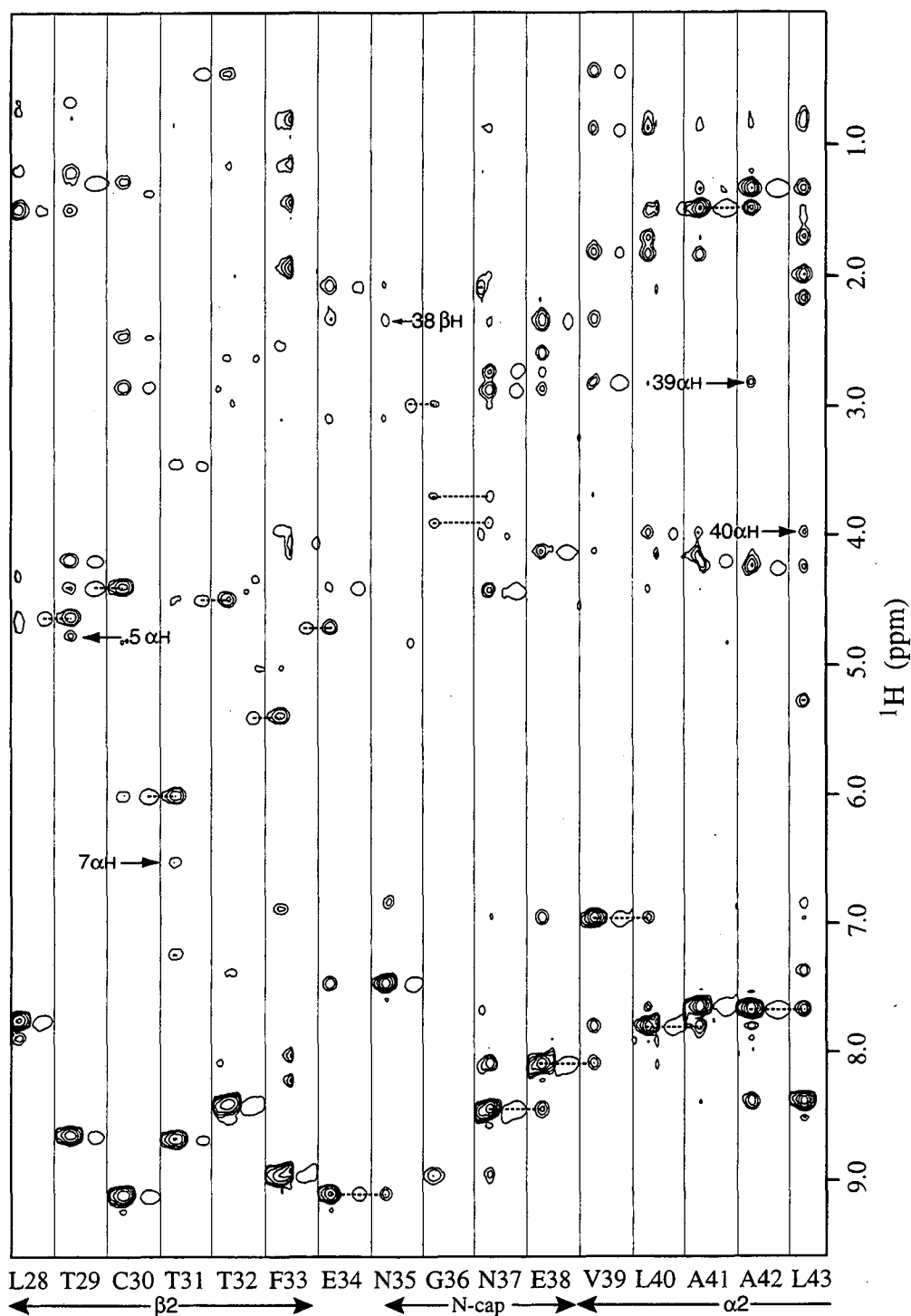
Figure 2.9: Strip plot of selected regions of the 3D ^{15}\text{N} NOESY-HMQC and TOCSY HMQC spectra of NTRC illustrating sequential resonance assignments for residues 28-43. NOESY and TOCSY strips are alternated with NOESY peaks displayed in multiple contours and the TOCSY peaks displayed with a single contour level. Sequential connectivities are indicated with dashed lines between NOESY and TOCSY peaks of sequential residues. Crosspeaks from 5 to 29 and 7 to 31 are due to cross-strand contacts in the \beta -sheet structure.
