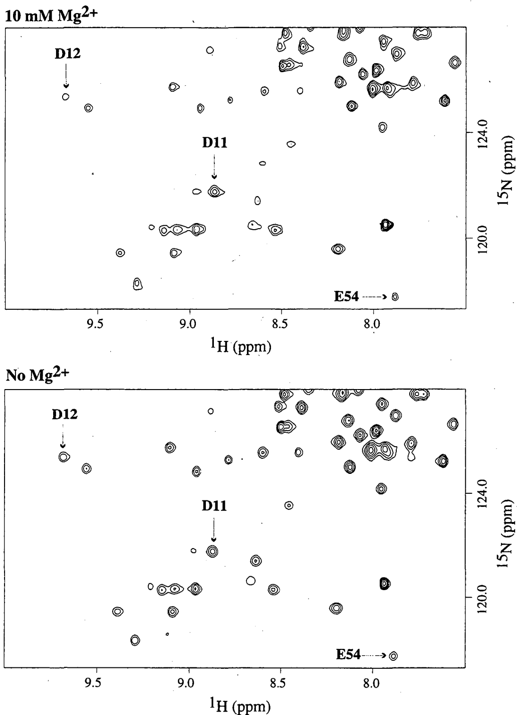
Figure 5.2: Sections of 1 H- 15 N HSQC's of D54E NTRC in the presence and absence of Mg 2+ . The positions of the active site residues D11, D12, and E54(D54) are indicated by arrows. The lack of change in these residues argues that D54E NTRC does not bind Mg 2+ at the active site.
