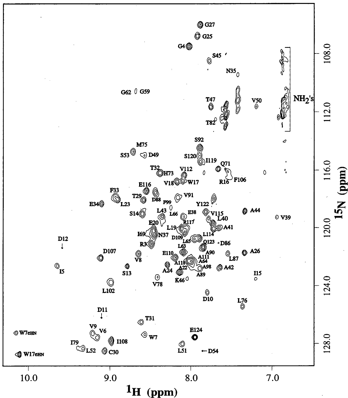
Figure 4.2: ^1\text{H} - ^{15}\text{N} HSQC spectrum of the receiver domain of NTRC in the presence of \text{Mg}^{2+} (1 mM NTRC, 10 mM sodium phosphate pH 6.4, 10 mM \text{MgCl}_2 ). Tentative crosspeak assignments, based on an assumption of minimal difference from apo-NTRC, are labeled. The arrows indicate the position of the active site residues D11, D12, and D54 in apo-NTRC.
