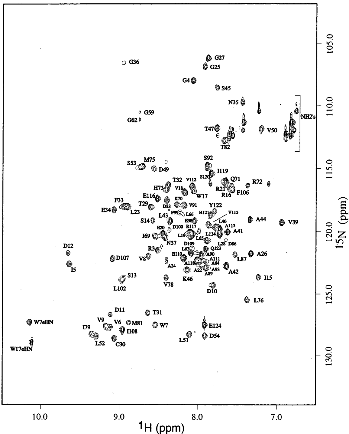
Figure 5.3: ^1\text{H} - ^{15}\text{N} HSQC of wild type NTRC (200 mM phosphate buffer pH 6.8). Assignments are indicated by the one letter amino acid codes and residue number. Note that there are very small rearrangements in this spectrum compared to that shown in Figure 2.8 due to differences in pH and buffer concentration.
