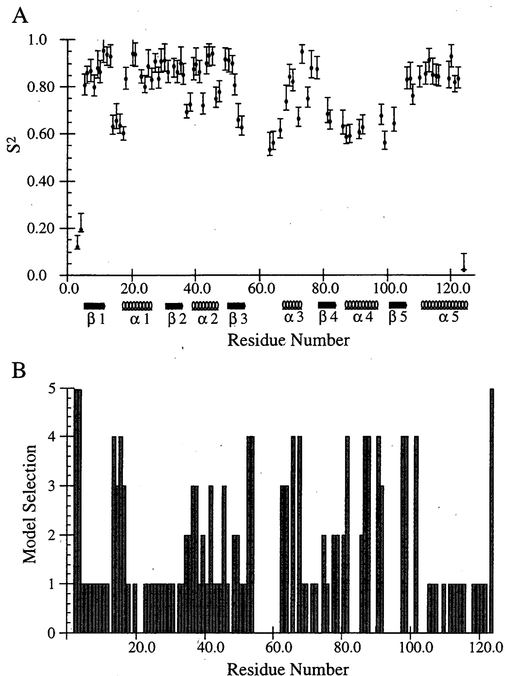
Figure 3.2: Model free parameters for the N-terminal domain of NTRC. Shown are (A) the order parameters for the backbone amides as a function of residue number and (B) The model of the spectral density used for analysis as a function of residue number. The models used (model 1-5) are described in the text. Note that a model selection of 0 indicates that complete relaxation data ( R_1 , R_2 and heteronuclear NOE) were not obtained for that residue.
