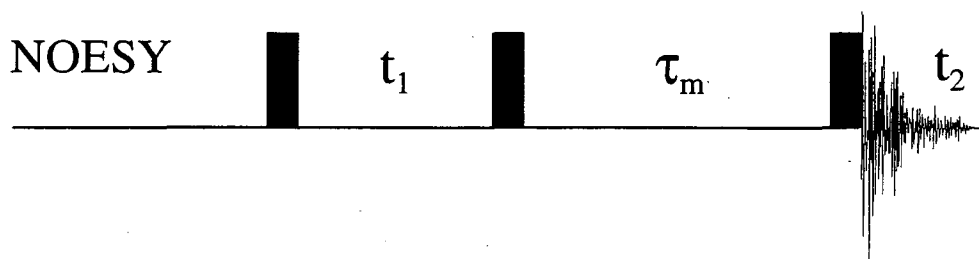
Figure 1.2: Schematic diagrams of 2D ^1\text{H} - ^1\text{H} pulse sequences. \pi/2 pulses are indicated with filled blocks. \tau_m is the the mixing time. See the text for details about these experiments.
