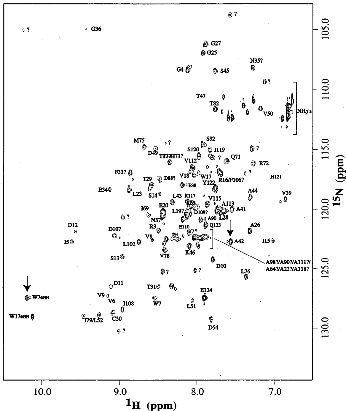
Figure 4.5: ^1\text{H} - ^{15}\text{N} HSQC spectrum of the receiver domain of NTRC under phosphorylation conditions (0.5 mM NTRC, 200 mM phosphate buffer pH 6.8, 300 mM carbamyl phosphate and 27 mM \text{Mg}^{2+} ). Tentative assignments, based on an assumption of minimal difference from unphosphorylated NTRC, are indicated. The arrows indicate peaks used for quantifying the degree of phosphorylation.
