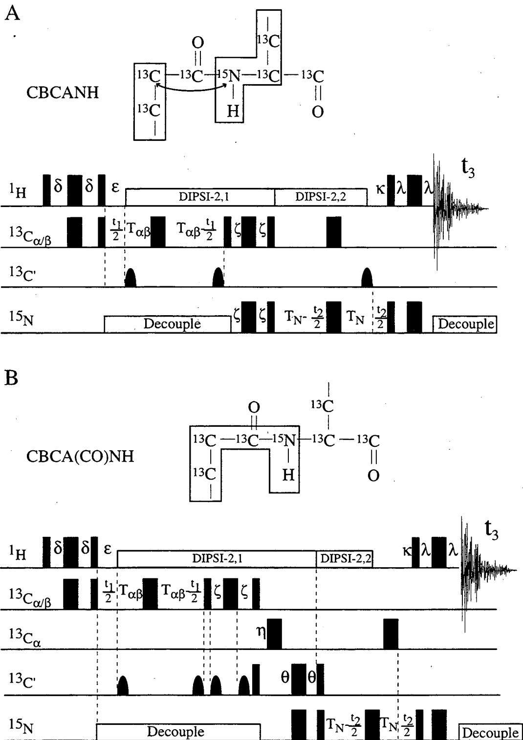
Figure 1.9: Schematic diagrams of the nuclei involved and the pulse sequences for the (A) CBCANH and the (B) CBCA(CO)NH. The delays \delta , \epsilon , \kappa , \lambda , and \zeta are set to maximize various INEPT type transfers. Details are given in the text.
