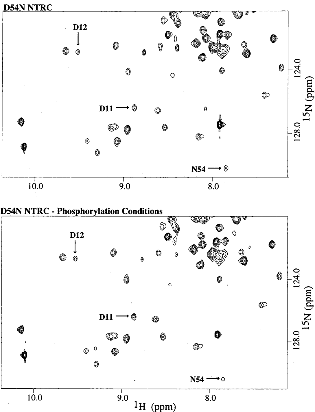
Figure 4.9: Sections of ^1\text{H} - ^{15}\text{N} HSQC's of D54N NTRC. The spectrum at the top was taken under non-phosphorylating conditions. The spectrum at the bottom was taken under phosphorylation conditions (the same as Figure 4.5). The lack of significant difference between the spectra indicates that phosphorylation at D54 is specific and responsible for the conformational changes seen in wildtype phosphorylated form of NTRC.
