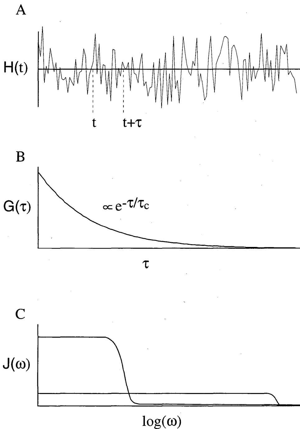
Figure 1.3: (A) A function randomly fluctuating in time. This is a model of the anisotropic interactions of a molecule rapidly tumbling in a liquid. (B) The autocorrelation function derived from a randomly fluctuating function as a function of \tau . This is an exponential decay with the correlation time, \tau_c , as characteristic time constant. (C) The spectral density function for two different correlation times.
