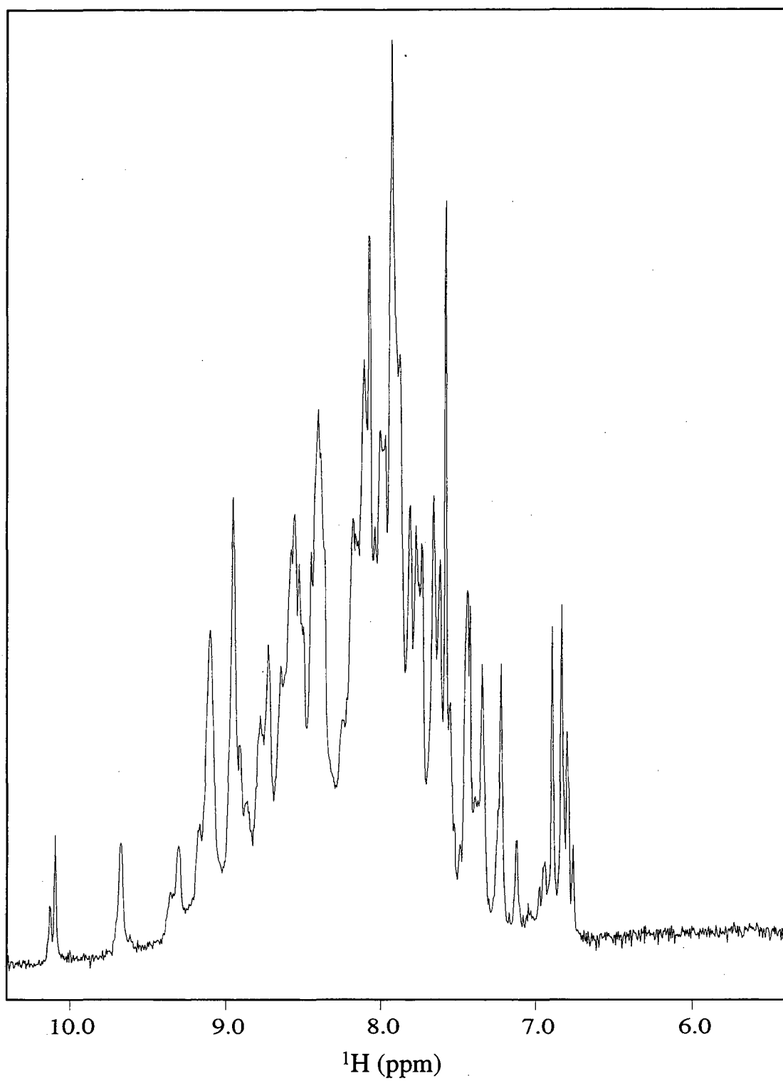
Figure 2.6: 1D ^1\text{H} spectrum of the amide region of the N-terminal receiver domain of NTRC at 600 MHz, pH 6.4, and 25°C.
