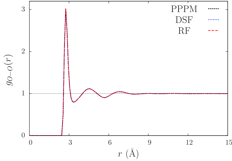
Fig. 2. Oxygen-Oxygen radial distribution function (RDF), g_{O-O}(r) , for SPC/E water using three different approaches to compute electrostatic interactions. Namely, particle-particle mesh (PPPM), damped shifted force potential (DSF) and reaction field (RF).
