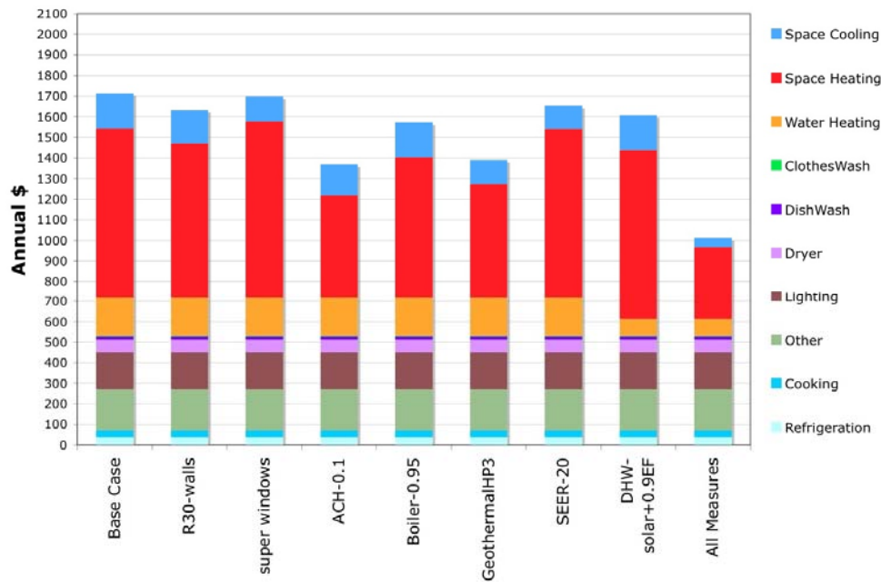
Figure 5: Effects of some simple standard efficiency measures
