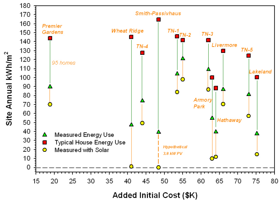
Figure 4: Plot of Cost vs. Measured Total Energy Use of a Compendium of Very Low Energy Homes. (Source: Parker . 2008)
