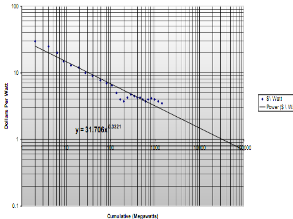
Figure 15: Log-Log Plot of Relationship Between $/Wp & Cumulative Megawatts Installed (1975-2000) (Source: Handleman 2000)
