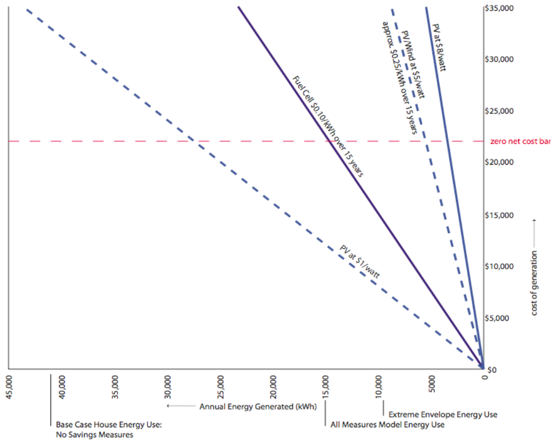
Figure 24: On-site Energy Generation Cost Curves
