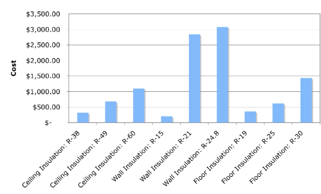
Figure 7: Average Incremental Cost per Home for Insulation
