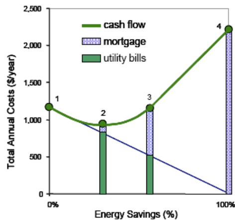
Figure 3: Conceptual plot of a least cost path to a ZEB, (from Anderson et al. 2004)
