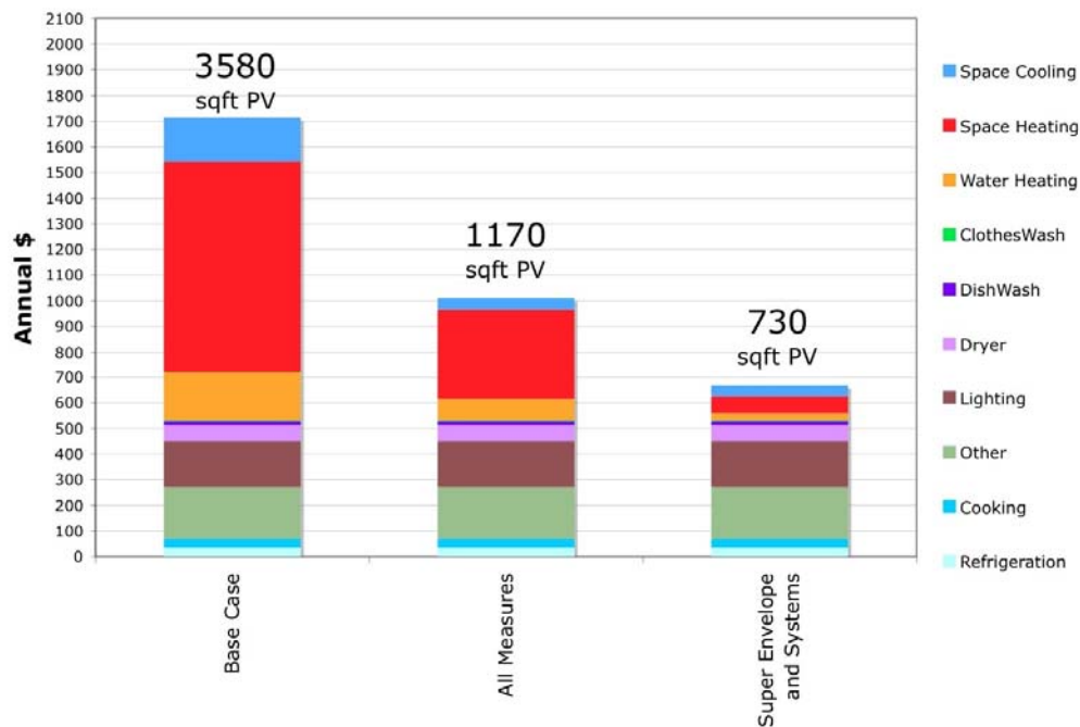
Figure 6: Some simple Zero Energy Variants of the Base Case home.
