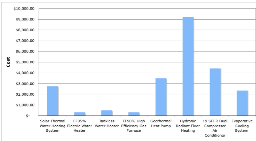
Figure 10: Average Incremental Cost per Home for HVAC & Water Heating
