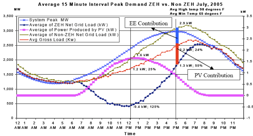
Figure 2: Average peak demand for Premier Gardens ZEB's vs. non-ZEB's, July 2005. (from Keesee, 2005)
