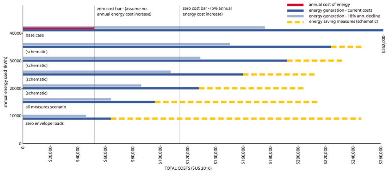
Figure 25: Energy Savings vs. Energy Generation Cost Curves (cost bar based on energy costs, unconverted to annual mortgage payments)
