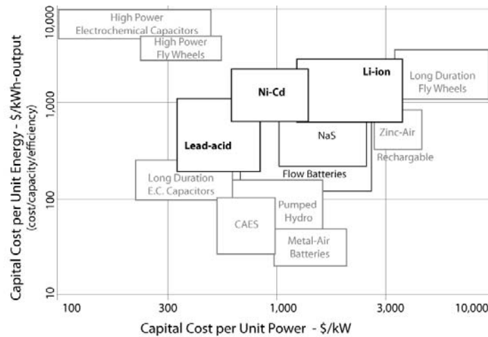
Figure 21: Energy/Power Storage Costs (Source Electricitystorage.org)
