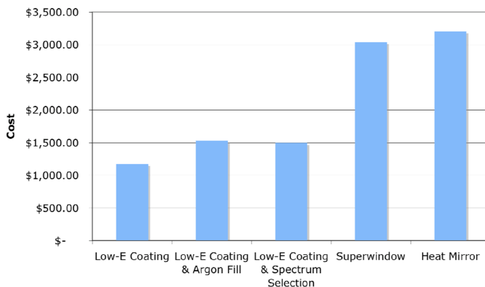
Figure 8: Average Incremental Cost per Home for Windows
