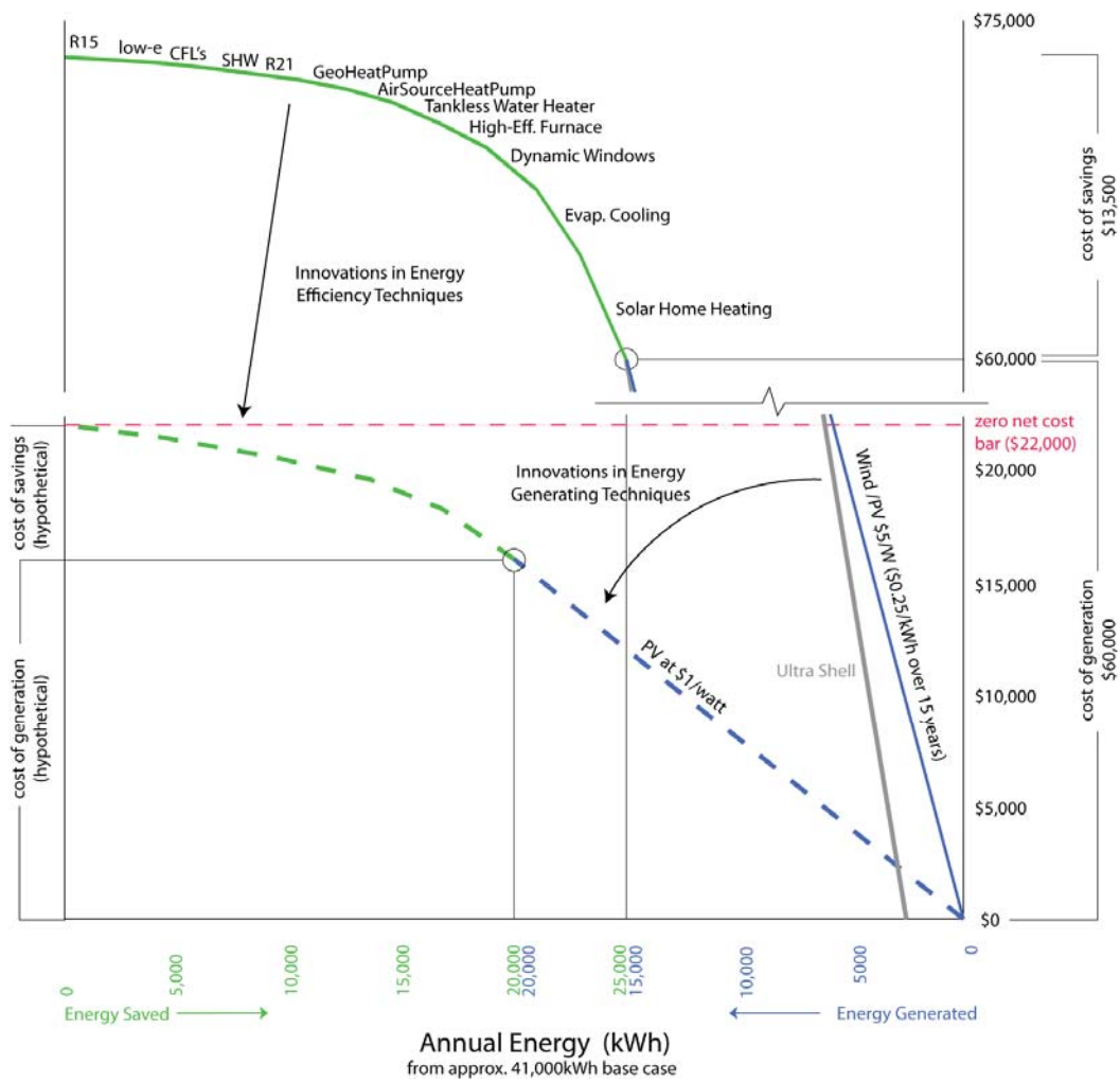
Figure 26: Energy Savings vs. Energy Generation Cost Curves, present technology and hypothetical innovations
