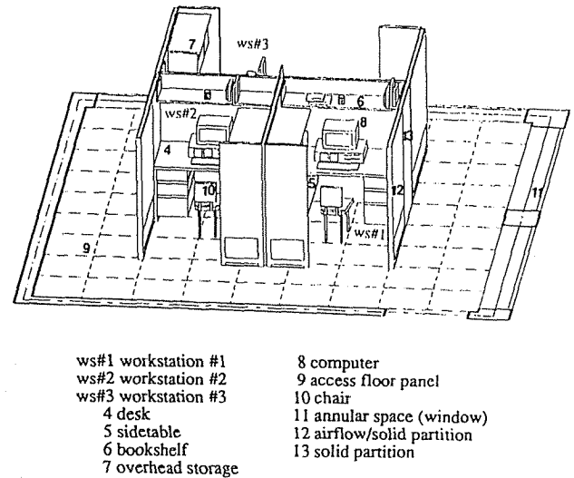
Figure 1b Chamber schematic.
