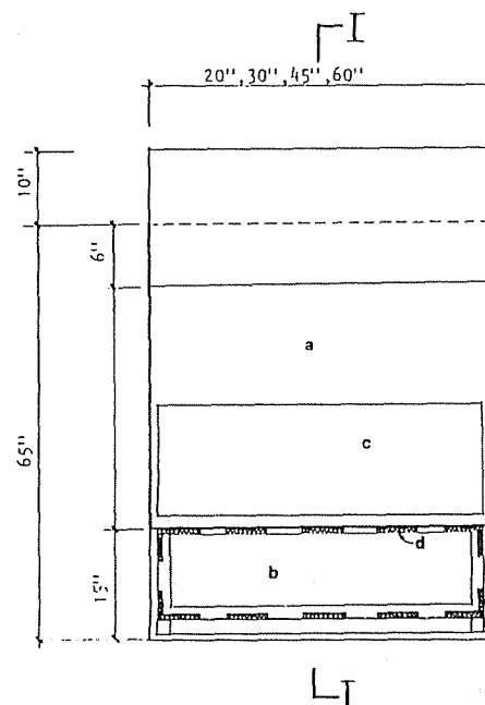
Figure 2 Partition configuration.
