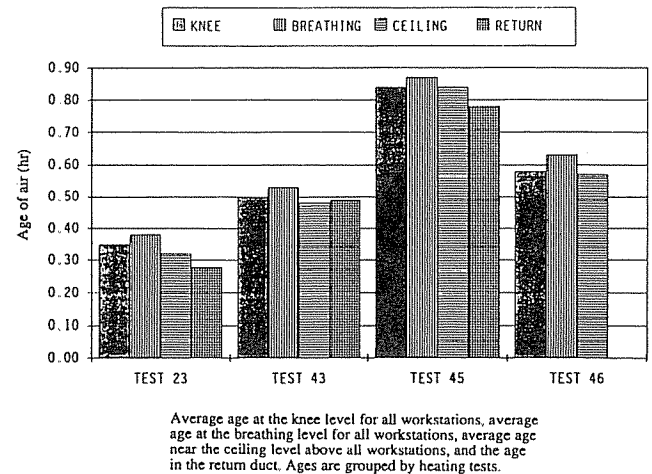
Figure 11 Variation in age of air with height.
