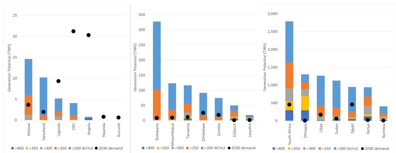
FIGURE 12: Wind generation potential (TWh) across the ACEC.
