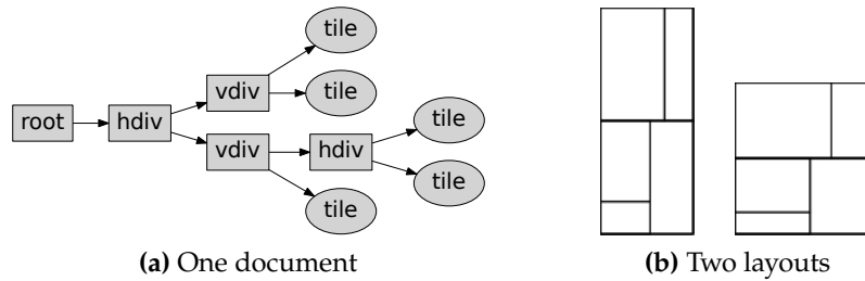
Figure 3.3.1. Debugging under-constrained languages. The two treemaps on the right have the same area but a different aspect ratio.
