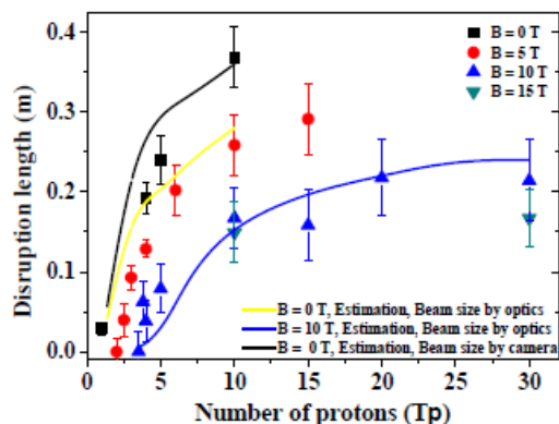
Figure 5: Disruption length vs. proton intensity.
