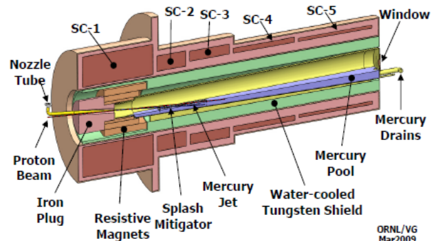
Figure 4: Hg-jet target concept studied in MERIT.
