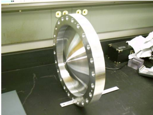
Figure 9: Thin aluminum window used for liquid-hydrogen absorber. The window and flange are machined at the University of Mississippi from a single disk, whose thickness in the center is reduced to 175 \mu\text{m} .
