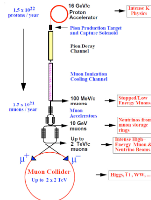
Figure 1: Schematic of MC subsystems.
