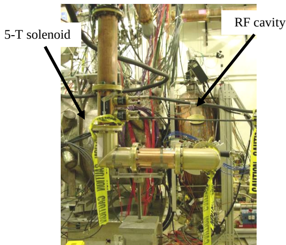
Figure 2: 201-MHz test cavity in the MTA.
