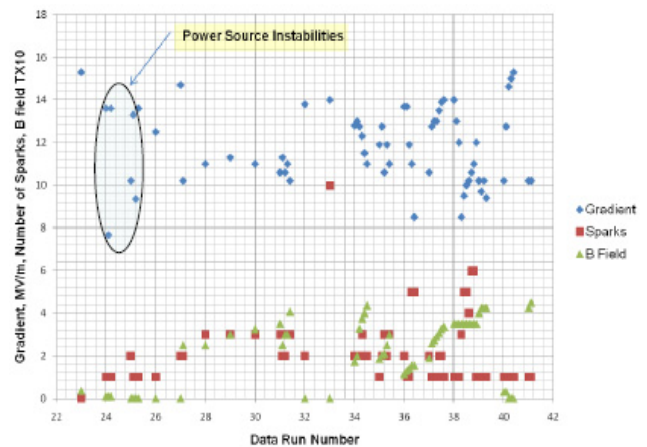
Figure 3: History of sparking during MTA magnetic field studies.
