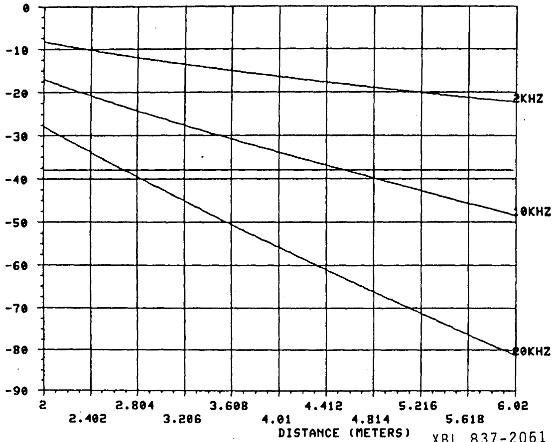
(DB) AMPLITUDE LOSS FOR FREQ=2,10,20 KHZ US-2500M/2 QS-20
