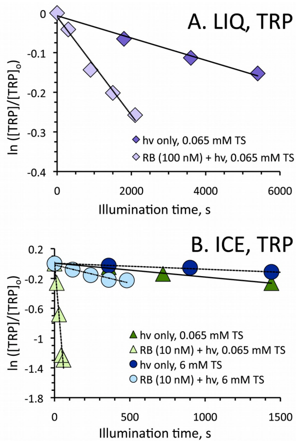
Figure 1. Loss of tryptophan (TRP) in liquid (A; 5°C) and ice (B; -10°C) samples both with an added sensitizer for ^1\text{O}_2^* (RB + hv) and without (hv only). All samples were illuminated with 549 nm light. Data for the regression lines are given in Supplemental Material, section S2.
