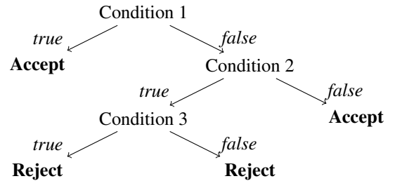
Figure 1: Example of a Fast-and-Frugal Decision Tree
