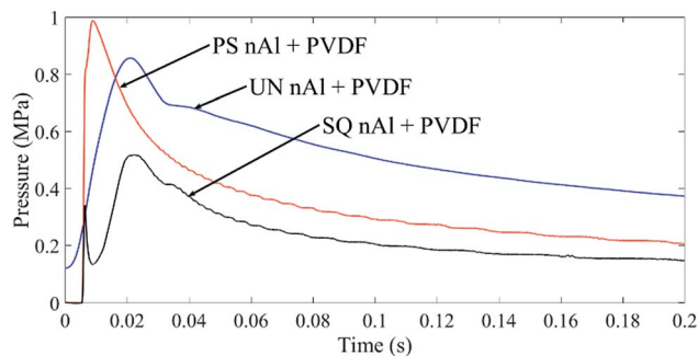
Fig. 3 Representative pressurization curves for untreated (UN), pre-stressed (PS), and super-quenched (SQ) nAl + PVDF films during impact ignition and combustion.
