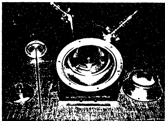
Fig. 3. Prototype longitudinal kicker with measurement wire.
