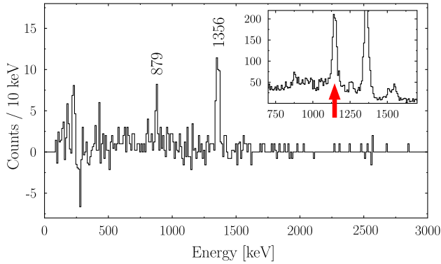
FIG. 2 (color online). The \gamma - \gamma coincidence technique was used to support the extraction of the level scheme. As an example, coincidences are shown when gating on the 1143 keV \gamma -ray transition (red arrow shown in the inset; same units as in Fig. 1).
