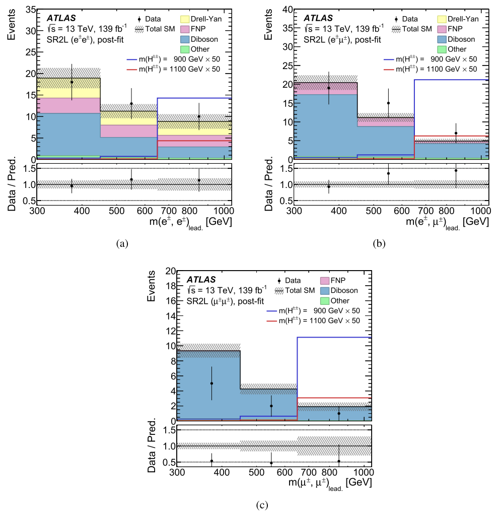
Fig. 6 Distributions of m(\ell^\pm, \ell^\pm)_{\text{lead}} in signal regions, namely a the electron–electron two-lepton signal region (SR2L), b the electron–muon two-lepton signal region (SR2L) and c the muon–muon two-lepton signal region (SR2L). The background expectation is the result of the background-only fit described in the text. The hatched bands include all systematic uncertainties post-fit with the correlations between various sources taken into account. The solid coloured lines correspond to signal samples, normalised using the theory cross-section, with the H^{\pm\pm} mass marked in the legend. The \times 50 in the legend indicates the scaling of the signal yield to make it clearly visible in the plots. The error bars show statistical uncertainties. Backgrounds from top-quark and multiboson processes are merged, forming the 'Other' category. The last bin also includes any overflow entries. The lower panels show the ratio of the observed data to the estimated SM background. The binning presented in the figures is used in the fit
