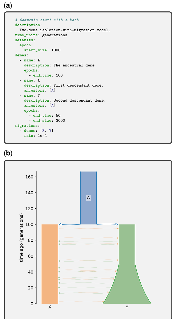
Fig. 1. Example isolation-with-migration Demes model. a) The HDM representation expressed as YAML. b) A visual representation of the model using demesdraw . The same model in the MDM form is provided in Fig. A1.
