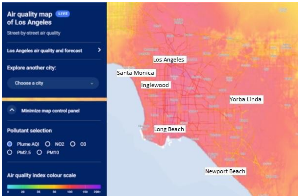
Figure 1. Plume Lab AQI levels for the Los Angeles region on January 28th, 2022. 34
