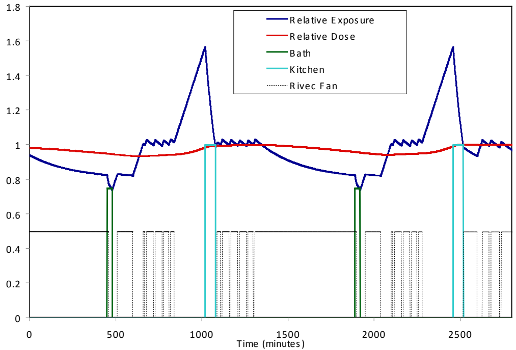
Figure 24. RIVEC operation for continuous supply in CZ3 in cooling season
