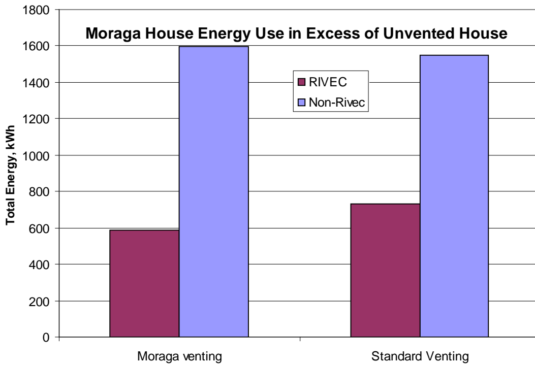
Figure 14. Simulated Total Energy Use of RIVEC and non-RIVEC ventilated homes relative to a house with no continuous mechanical ventilation.
