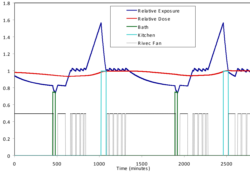
Figure 20. RIVEC operation for continuous exhaust in CZ3 in cooling season
