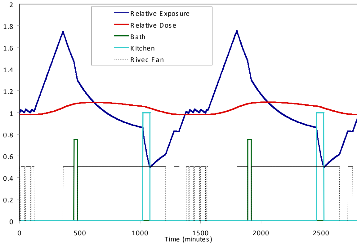
Figure 18 Illustration of RIVEC fan operation (CZ3 heating)
