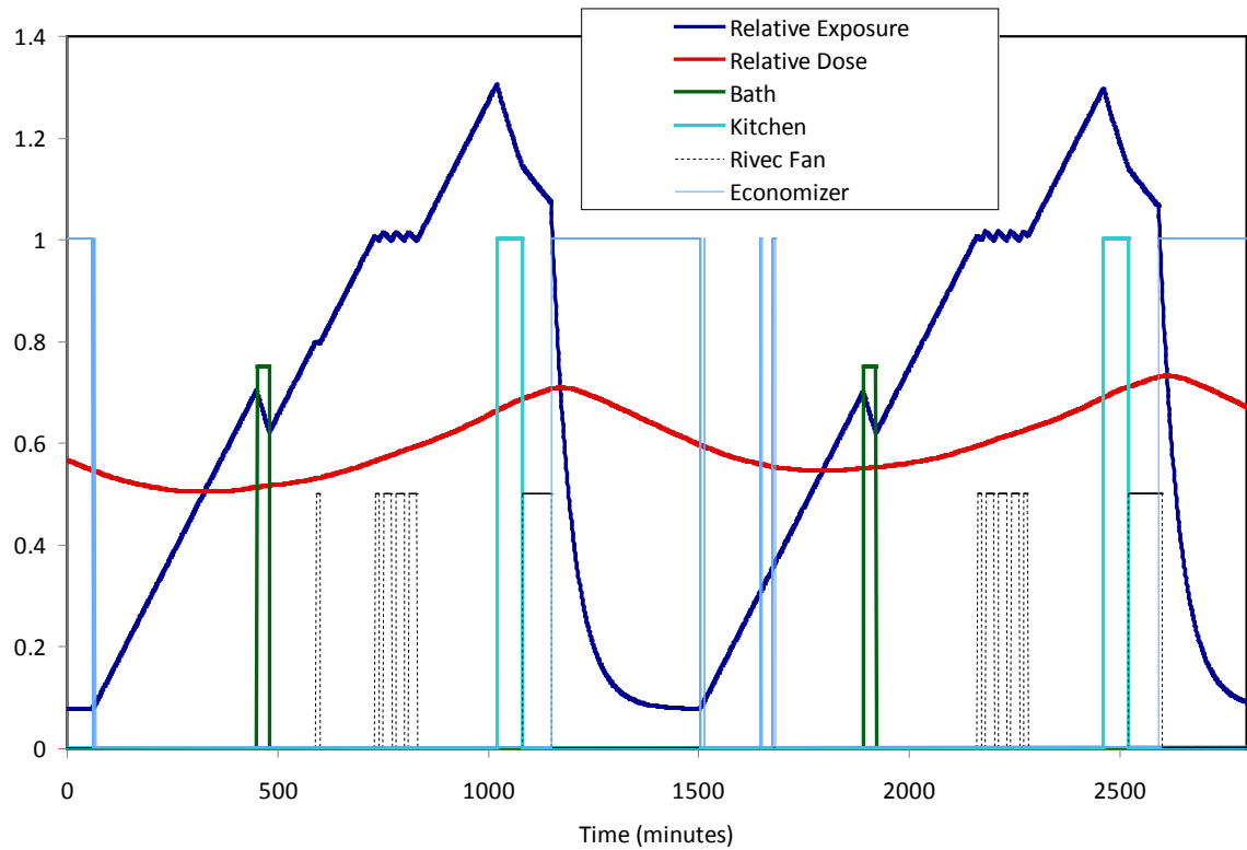
Figure 9. Standard fan schedule RIVEC operation for cooling in Moraga house
