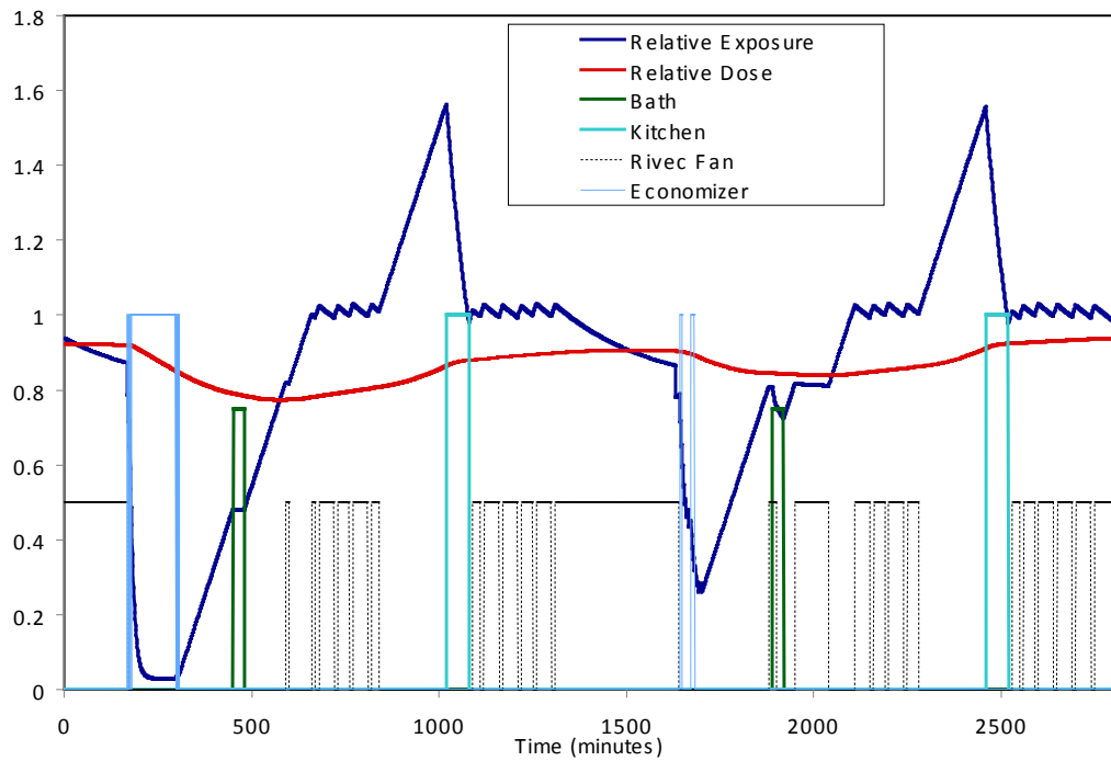
Figure 25. RIVEC operation for continuous exhaust + economizer in CZ13 in cooling season
