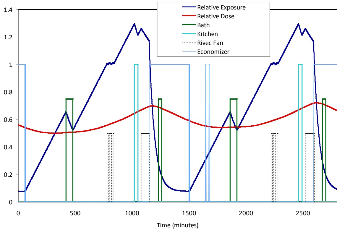
Figure 8. Moraga fan schedule RIVEC operation for cooling
