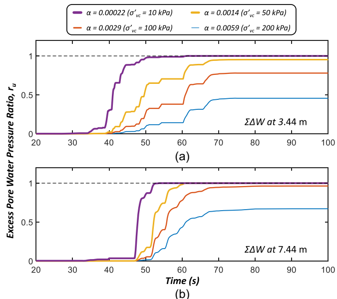
Fig. 11. Sensitivity analysis of coefficient \alpha corresponding to the effective stress of 10, 50, 100, and 200 kPa: (a) the depth of 3.44 m; and (b) the depth of 7.44 m.
