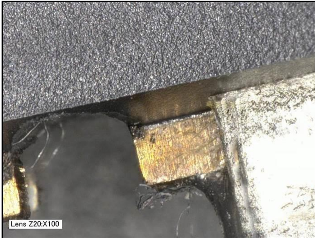
Figure 8-3: Metallic Whiskers (courtesy 3M)
