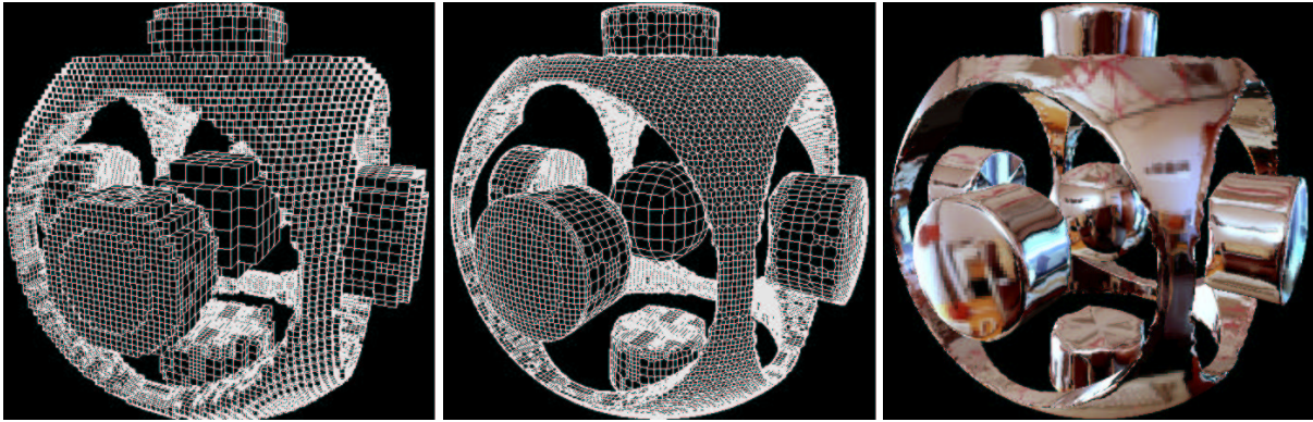
Fig. 1. Topology changes of sphere created by sweeping tori through it: octree cells (left), resulting mesh (middle) and high-quality rendering using environment mapping.
