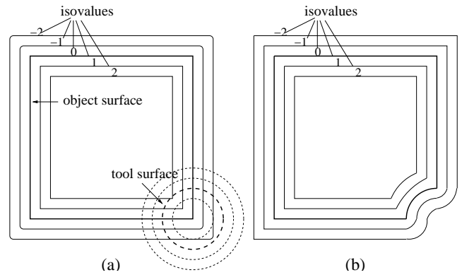
Fig. 2. Isolines of a distance field before (a) and after carving operation (b).
