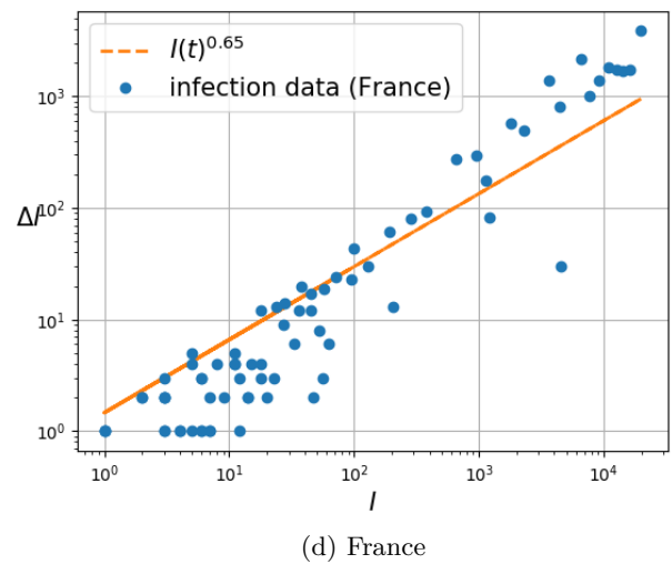
Fig. 8: Relationship between infection growth \Delta I(t) and the number of infected individuals I(t) with COVID-19 in four different countries.
