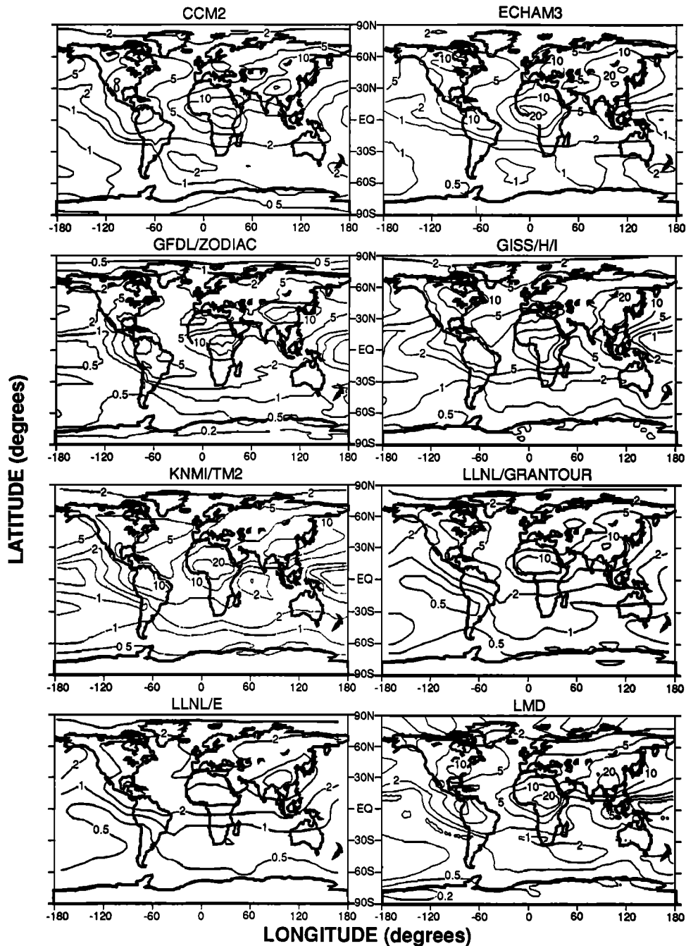
Figure 4. Mean 222 Rn concentrations simulated by the different models at 300 hPa in June-August. Units are 1 x 10 -21 mol/mol; see text for conversion factors.
