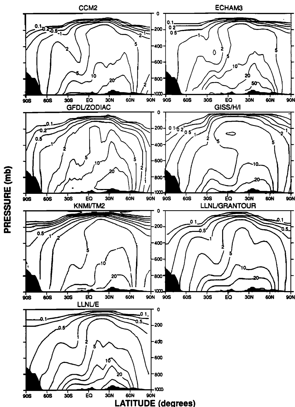
Figure 5. Zonal mean 222 Rn concentrations (units of 1 \times 10^{-21} mol/mol) simulated by the different models in June-August.
