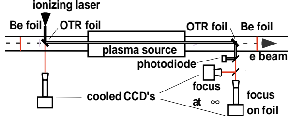
FIG. 1. Experimental setup
