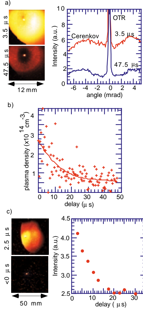
FIG. 4. Downstream foil data are shown for two wavelength ranges: (a-b) 676.4 nm (1.35 m oven) and (c) 505 nm (1 m oven). a) Images at high ( 3.5 \mu\text{s} delay) and low ( 47.5 \mu\text{s} delay) plasma density. Lineouts show inward shift of CR cone and increase in visible background level. b) Plasma density estimated from inward shift of CR cone angle vs. delay. c) Images at \Delta t < 0 and 2.5 \mu\text{s} delay show spatial extent of background and total intensity collected into 80 nm BW vs. delay. The edge in the image taken at 2.5 \mu\text{s} delay is due to the 2'' pellicle aperture.
