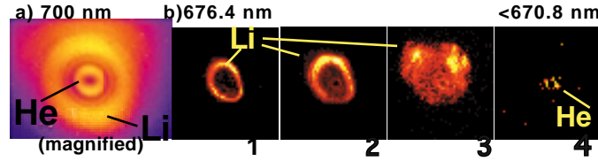
FIG. 2. a) Far field image (537 °C) shows separate cones for the Li and He regions. b) Far field wavelength scan from 676 nm through and below the resonance shows disappearance of Li CR cone, and trends in cone radius and width. Wavelength decreases from left to right. Dispersive effects have broadened the cone radius and width in frame 3. The asymmetry in (b) is due to the surface irregularity of a splitting pellicle added to the system.
