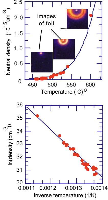
FIG. 3. a) Neutral density estimated from CR and b) its functional dependence are plotted for an oven cool down. The solid lines are known vaporization curves [15].
