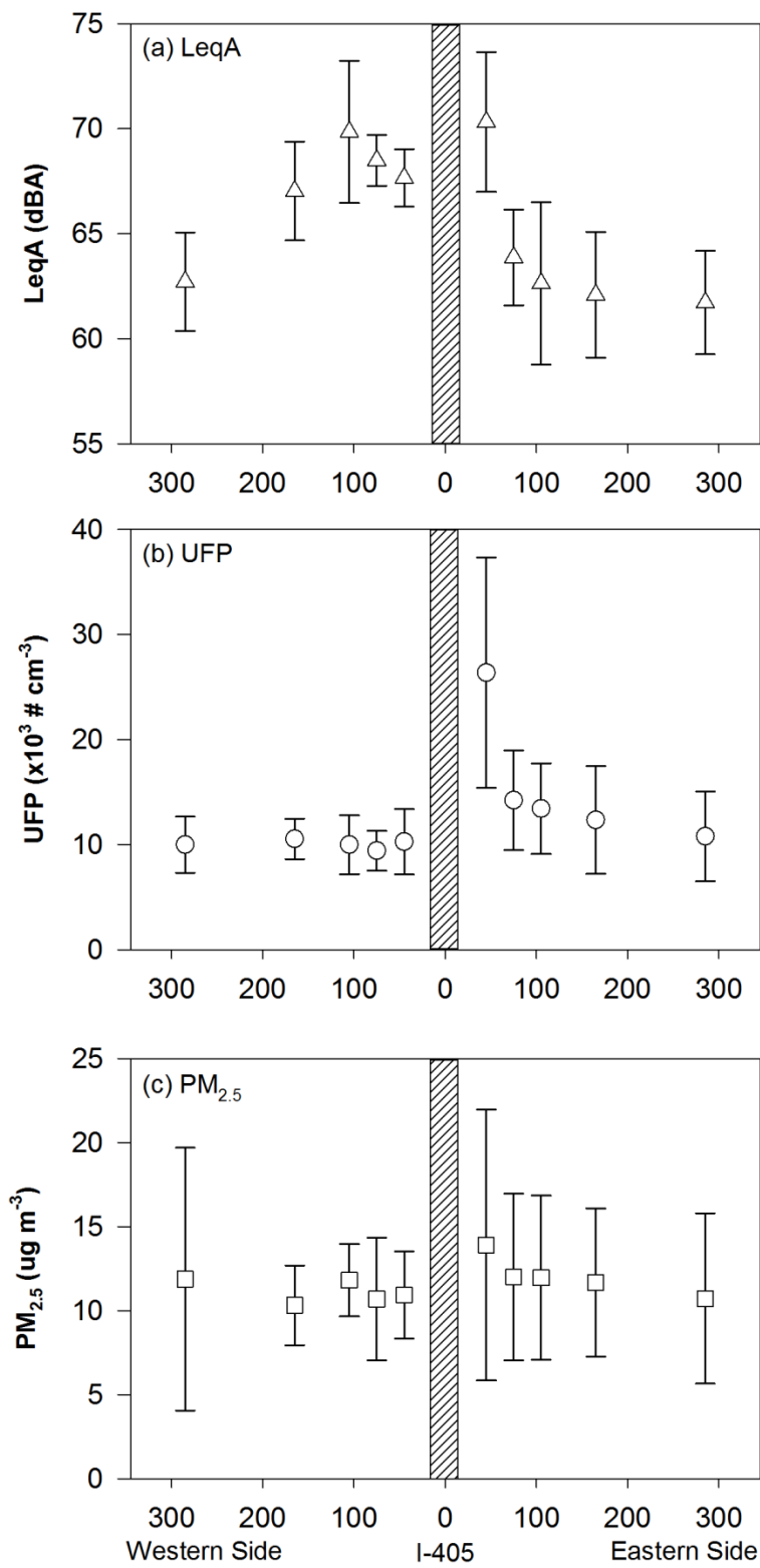
Figure 7. Noise level, ultrafine particles number concentration, and \text{PM}_{2.5} mass concentration measured along Constitution Avenue.
