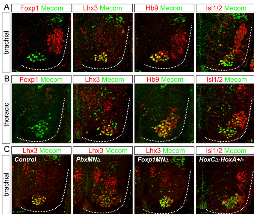
Figure 7. Hox-Independent Regulation of Mecom by Pbx Proteins and Lhx3
