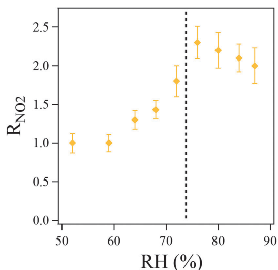
Fig. 2 Rates of \text{NO}_2 release in \text{NaNO}_3 photolysis experiments as a function of RH. The vertical dashed line is the \text{NaNO}_3 DRH. Error bars are 2s of duplicate experiments.
