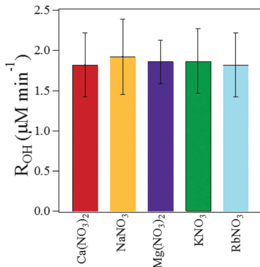
Fig. 3 The rate of OH production in bulk-phase photolysis studies conducted at 313 nm and 298 K. Error bars are 2σ of triplicate experiments.
