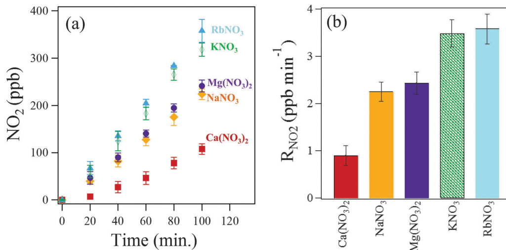
Fig. 1 (a) \text{NO}_2 production during photolysis experiments for aqueous thin films of \text{Ca}(\text{NO}_3)_2 (red, squares), \text{NaNO}_3 (orange, diamonds), \text{Mg}(\text{NO}_3)_2 (purple, circles), \text{KNO}_3 (green open diamonds) and \text{RbNO}_3 (blue, triangles), and (b) the corresponding rates of \text{NO}_2 production at 298 K in air. Hatched bars and open symbols for \text{KNO}_3 denote experiments conducted below the DRH. Error bars are 2s of triplicate experiments.
