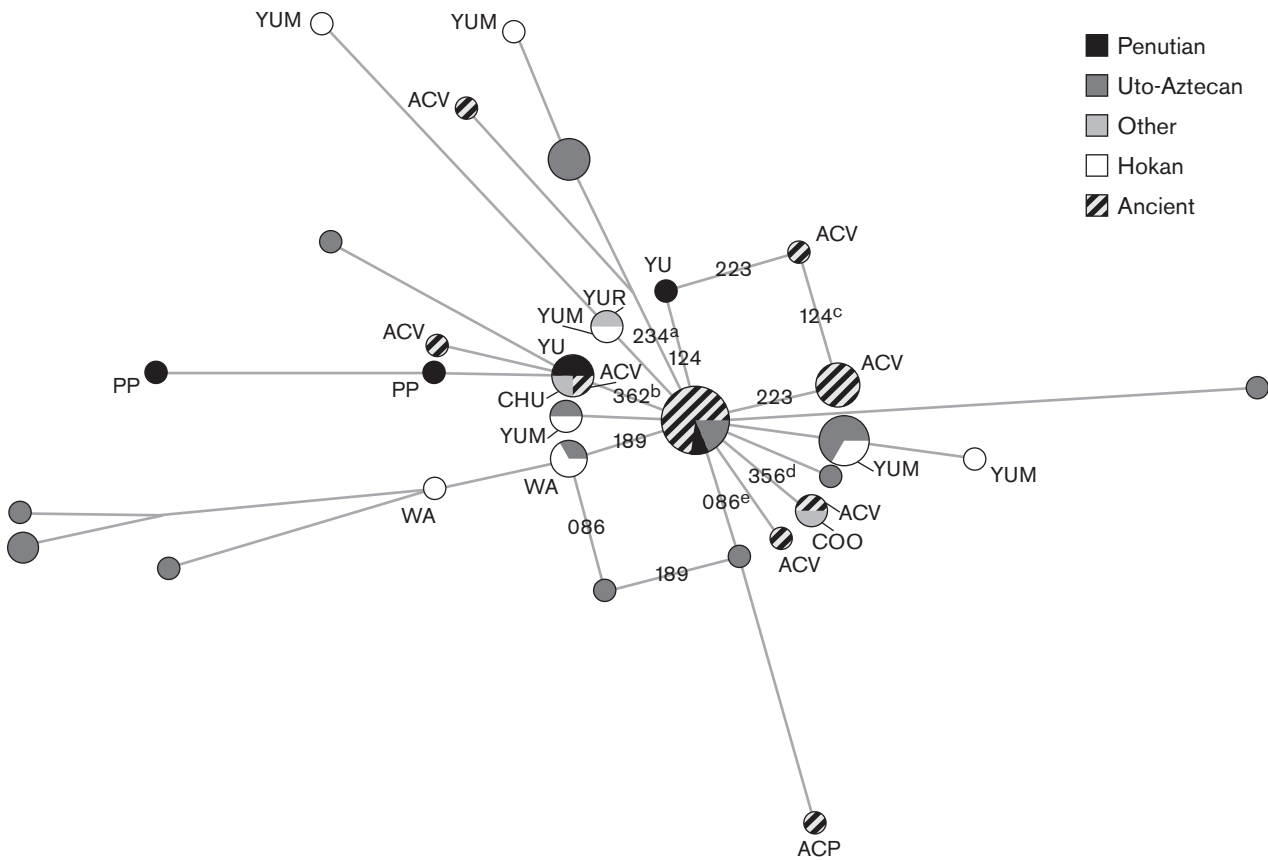
Figure 5. Haplogroup C network. WA = Washo, YUM = Yuman, YUR = Yurok, COO = Coosan, PP = Plateau Penutian, YU = Yok-Utian, CHU = Chumashan, ACP = Ancient Columbia Plateau, ACV = Ancient Central Valley, AGB = Ancient Great Basin. The basal C node includes two Uto-Aztecan (one Numic and one Takic), one Plateau Penutian, six Ancient Central Valley, one Ancient Columbia Plateau, and one Ancient Great Basin sample. One lineage observed solely in the Washo that is two mutations away from basal C was removed from the network because of lack of space.
