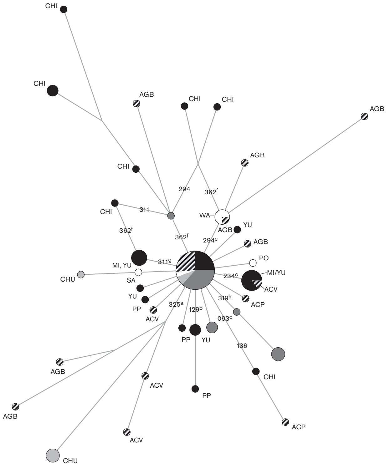
Figure 6 . Haplogroup D network. PO =Pomoan, SA =Salinan, WA=Washo, CHI=Chinookan, PP =Plateau Penutian, MI =Maiduan, YU=Yok-Utian, CHU =Chumashan, ACP=Ancient Columbia Plateau, ACV=Ancient Central Valley, AGB=Ancient Great Basin. The basal D node includes four Uto-Aztecan (two Numic, one Takic, and one Tubatulabal), five Yok-Utian, two Chumashan, five Ancient Central Valley, and two Ancient Great Basin samples.
