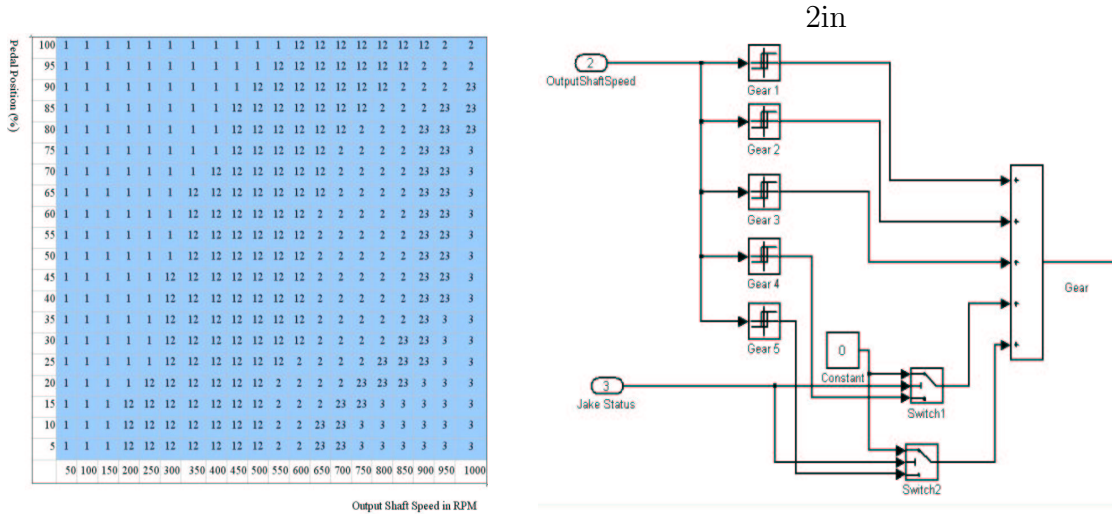
Figure 1.4: Part of acceleration shift scheduleFigure 1.5: Deceleration shifting implementation
