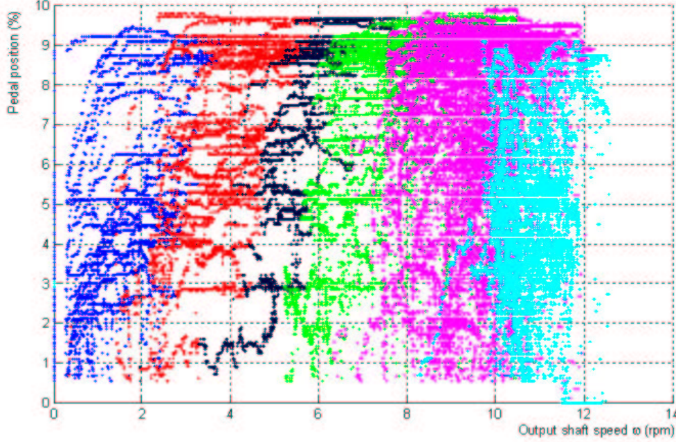
Figure 1.1: Shifting Data - Experiment: Blue-Gear 1; Red-Gear 2; Black-Gear 3; Green-Gear 4; Magenta-Gear5; Light blue-Gear6
