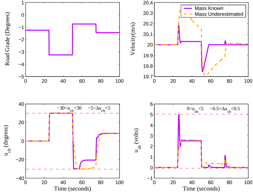
Figure 4.4: Velocity regulation when vehicle mass is underestimated.
