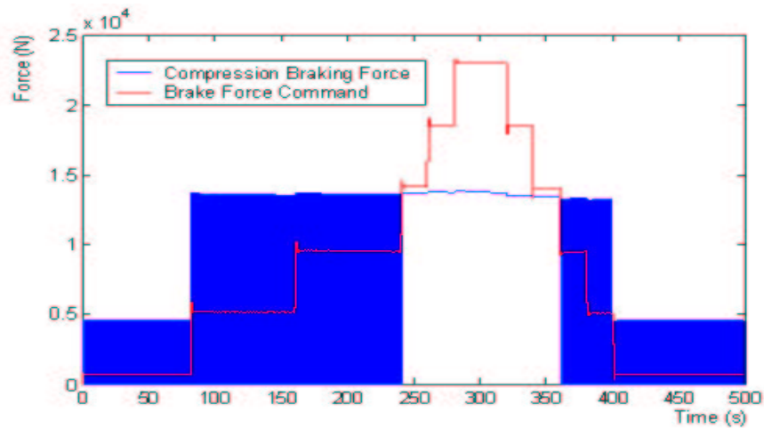
Figure 2.8: Compression brake usage: PWM actuation
