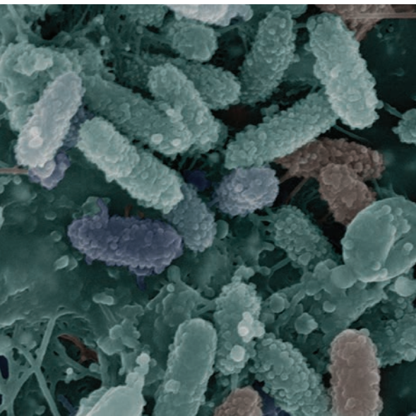
PRECIPITATION OF TOXIC SELENIUM OUT OF GROUNDWATER BY MICROORGANISMS
