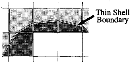
Figure 19: A infinitely thin shell geometry. Cell fragments can be generated along both sides of a polyline; our schemes support multiple cell fragments at a given mesh cell index.
