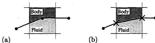
Figure 16: The two methods used in this paper for computing cell fragments. (a) The “natural” method: Compute the cell fragment according to the specified polygon, exactly. (b) The “blunted” method: Compute the cell fragment using the grid line intersection locations. The blunted method only builds cells that are exactly discretized by the finite-volume conservation sum. The piecewise-linear boundary interfaces allowed by the natural method are only approximated by the flux sum.
