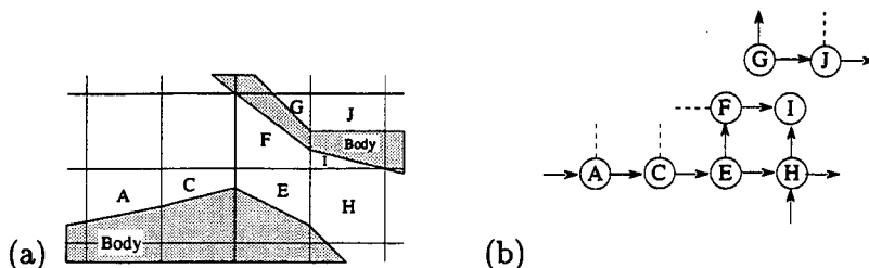
Figure 7: (a) A small region of a typical multiply-connected geometry. Cells A, C, F and J are bounded on a side by “interface” faces. (b) The graph representation of the partial cells labeled in (a). The dotted lines indicate interface faces, which are not strictly part of the graph. Information from the logically rectangular data communicates with the graph via the interface faces.
