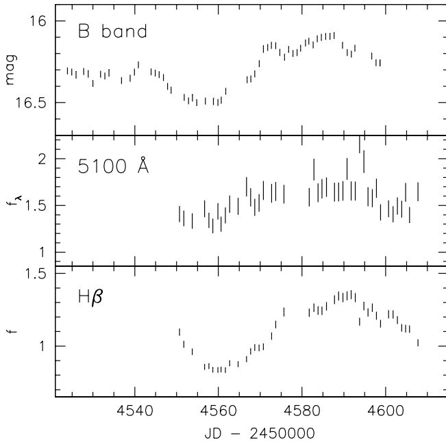
FIG. 1.— Light curves for Arp 151. From top to bottom, the panels are: B -band magnitude, observed continuum flux density at rest-frame 5100 Å, and H \beta emission-line flux. The units are as given in Table 1 for 5100 Å and H \beta .
