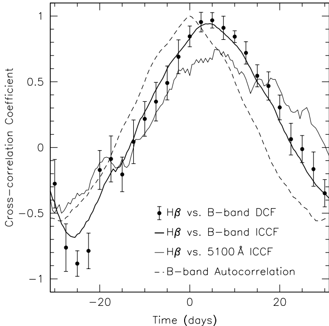
FIG. 3.— Cross-correlation functions for Arp 151. The heavy line is the cross-correlation of the B -band flux and H\beta emission, and the data points show the discrete correlation between the same. The cross-correlation of the 5100 \text{ \AA} flux and H\beta (thin solid line), while noisier, is consistent. The dashed line is the B -band auto-correlation function, which peaks at zero lag as expected.
