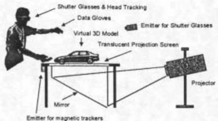
Figure 1: Hardware setup.
