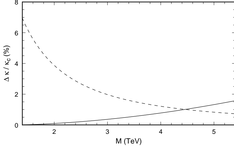
Figure 4: The amount of fine-tuning required 23 in the TC^2 model. The dashed line is the amount of fine-tuning in \Delta\kappa_{eff} required to keep m_t much lighter than M , see equation (5.10). The solid curve shows the amount of fine-tuning (see equation (5.9)) in \Delta\kappa_{tc} required to satisfy the bound \Delta\rho_* < 0.4\% . The region excluded by the experimental constraint on \Delta\rho_* is above the solid curve.
